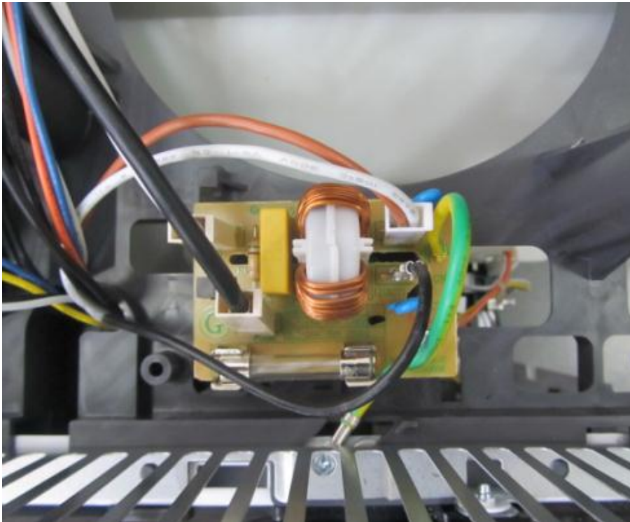
Power Filter Board- Top View
