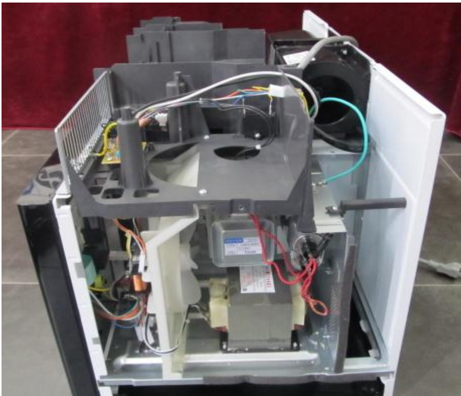
EUT Uncovered View
