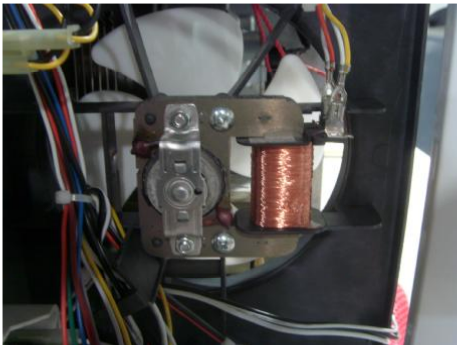
EUT-Inside View#2
