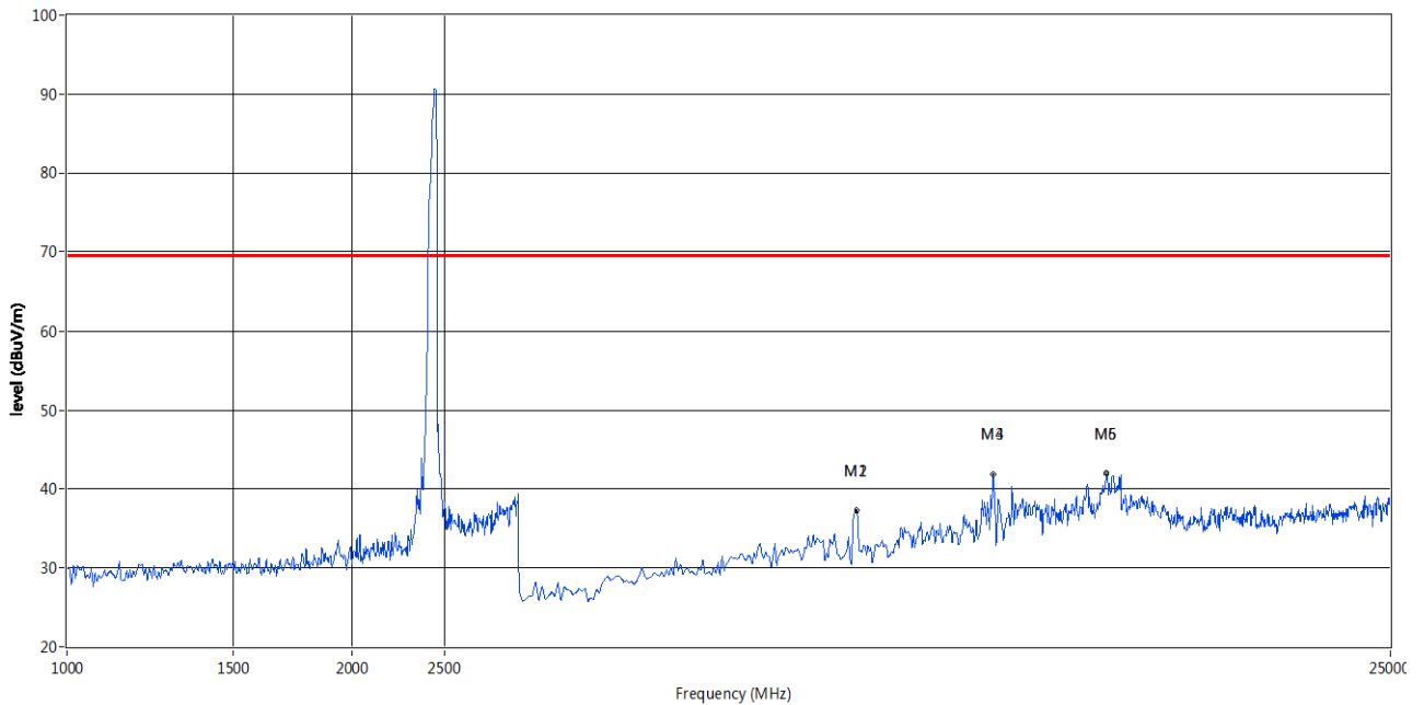
RE_EN Test Case_FCC 18 1GHz-25GHz
