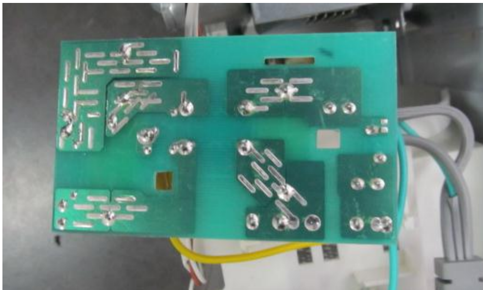
Power Filter Board Bottom View
