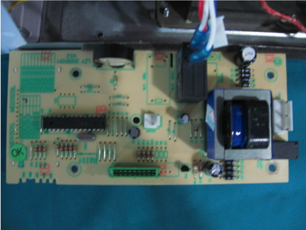
Main board #1
