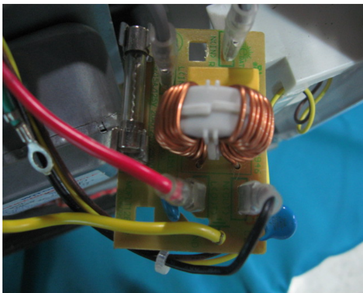
Photo 2- Front view of AC Power filter board
