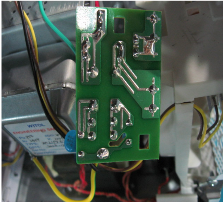
Photo 3 – Back view of AC Power filter board
