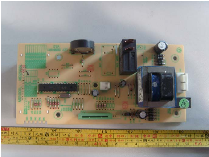
Main Board #1
