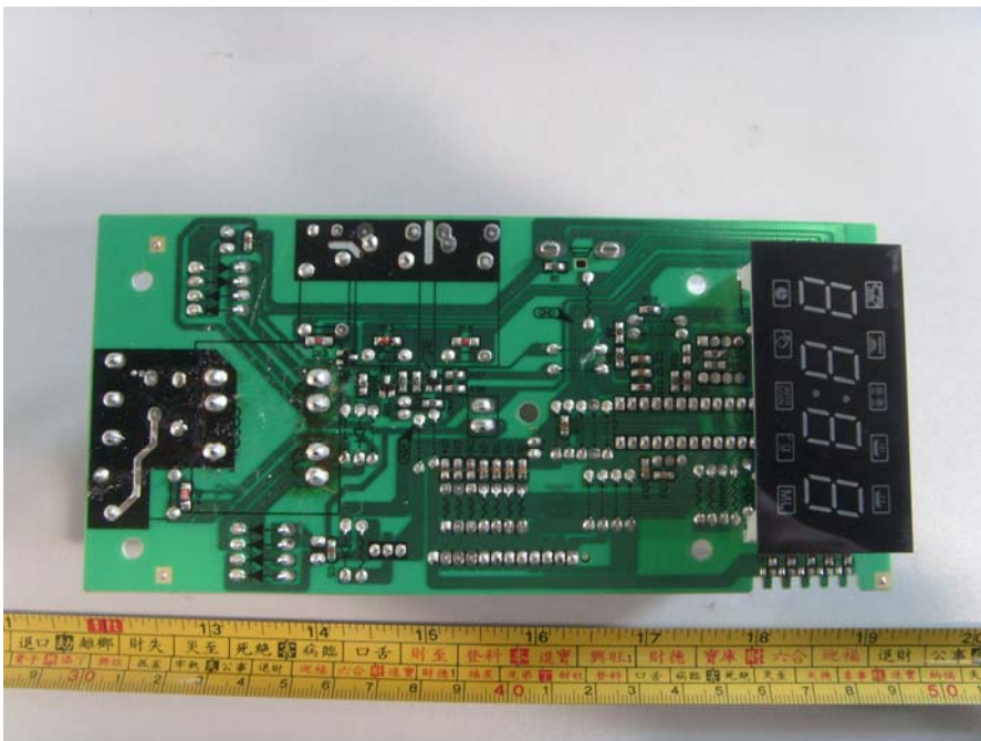
Main Board #2
