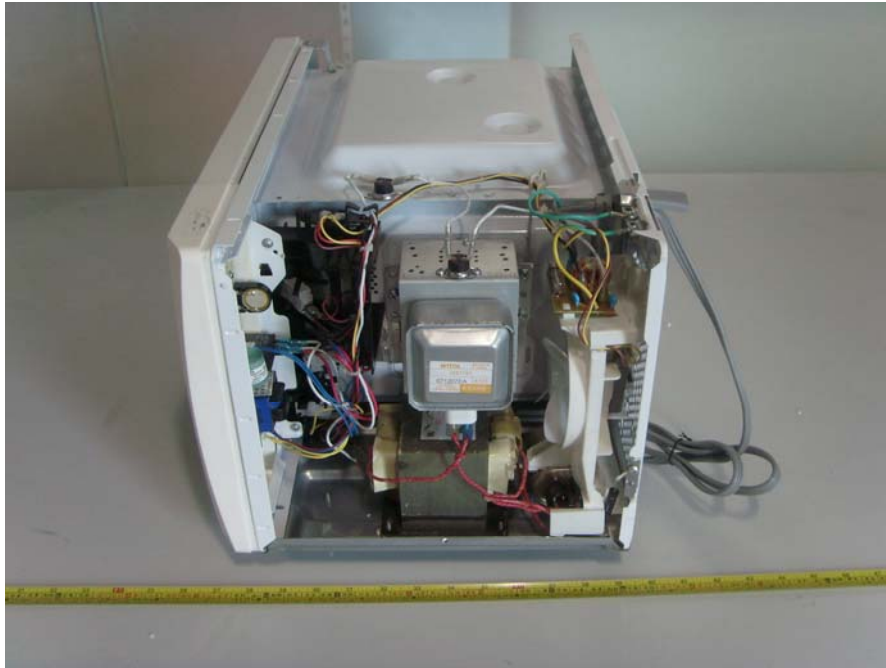
Inside View #1
