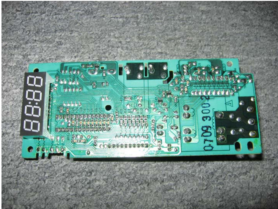
Main board #2
