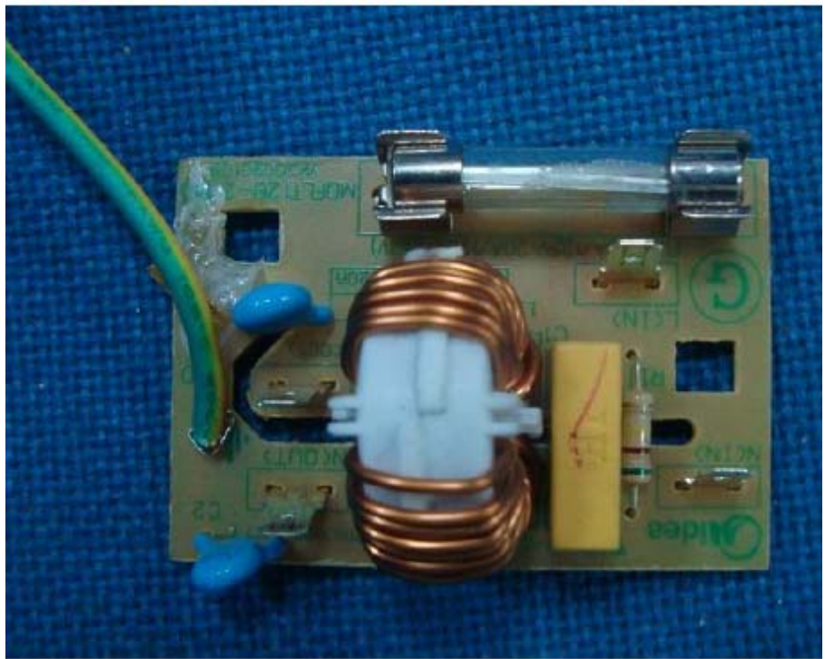
Power Filter Board -Front View
