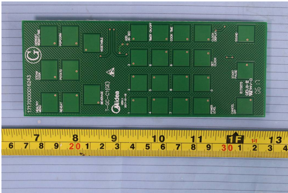
EUT – Control Panel Top View
