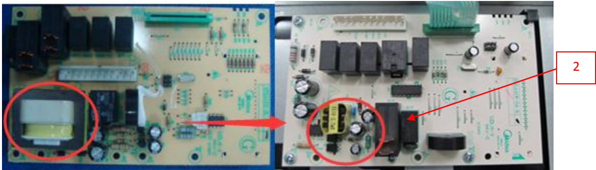
Original Mother board-top view
