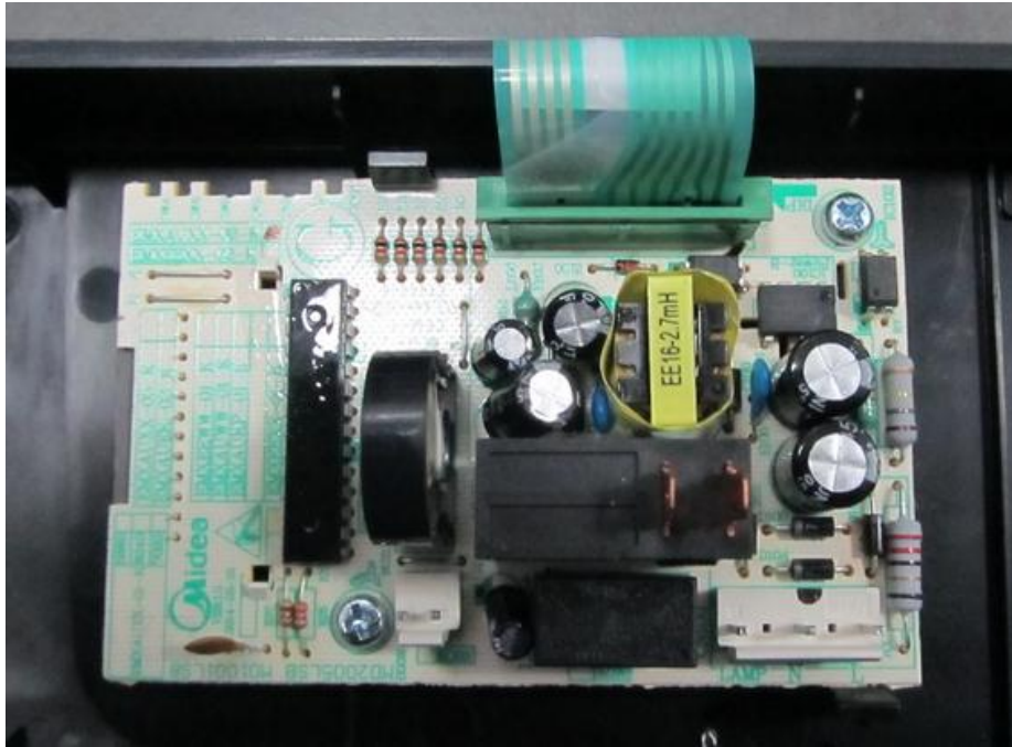
Mother board #1 Top View
