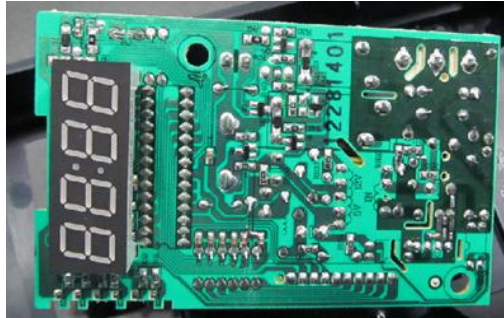
New Mother board -bottom
