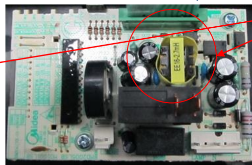
New Mother board –top view
