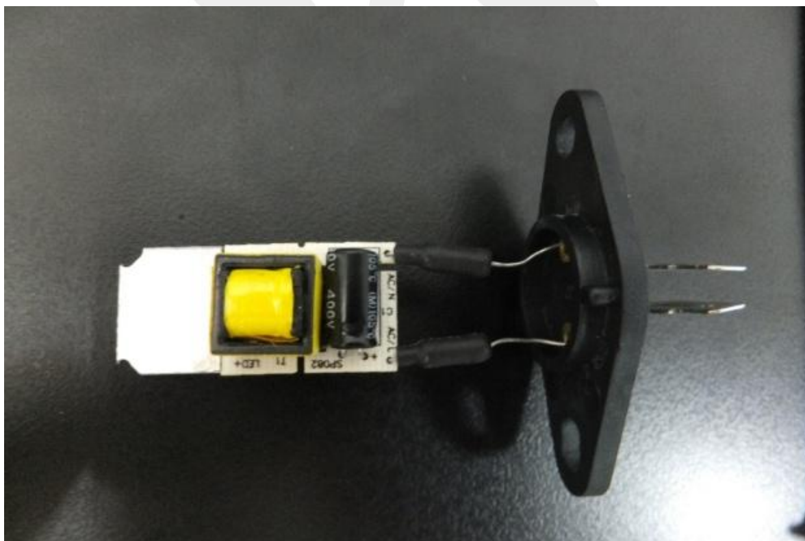
LED Lamp 2: PCB board- Top View
