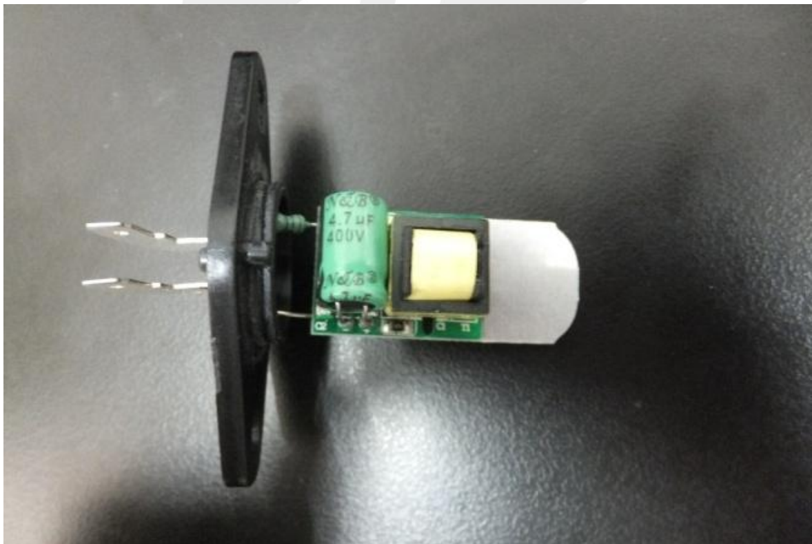
LED Lamp 1: PCB board- Top View
