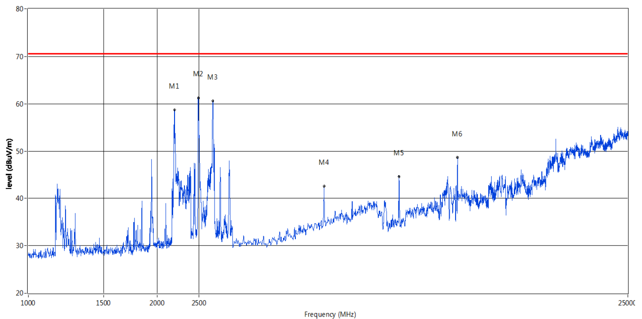
RE_EN Test Case FCC 18 1GHz-25GHz
