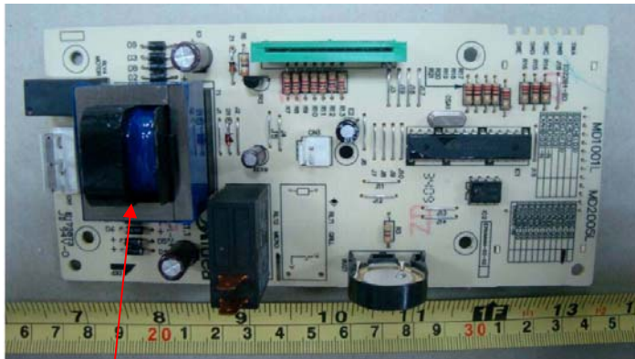
New mainboard
