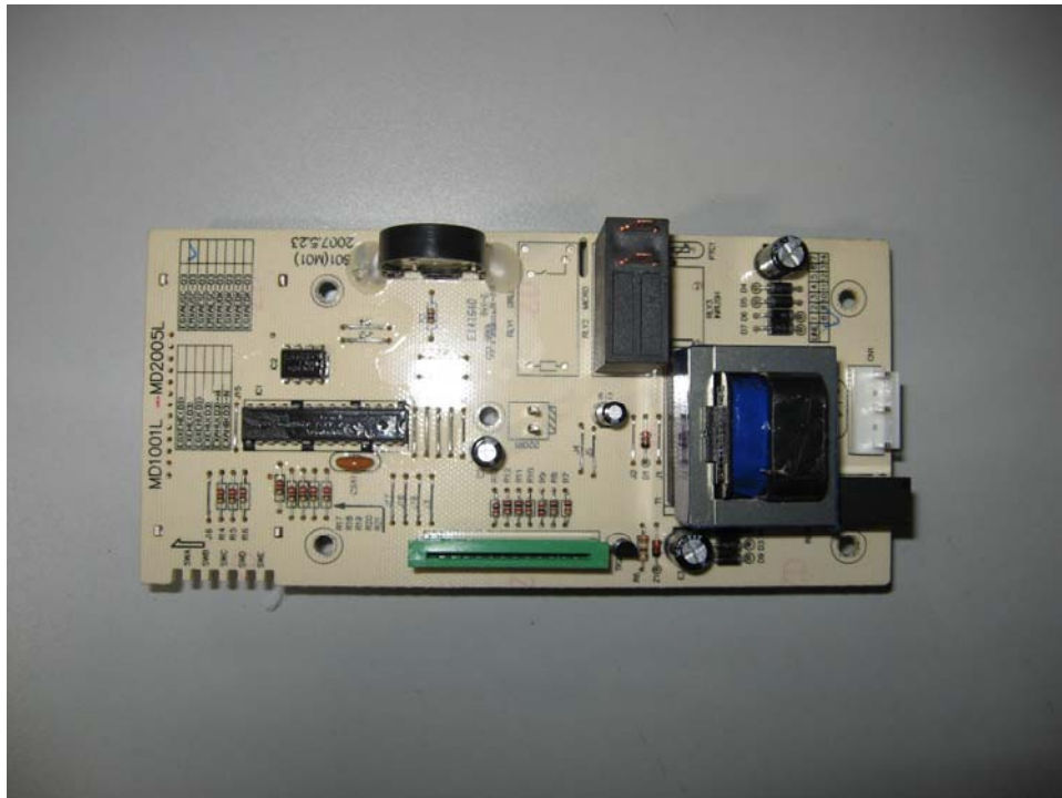
Photo 3 - Top view of main board
