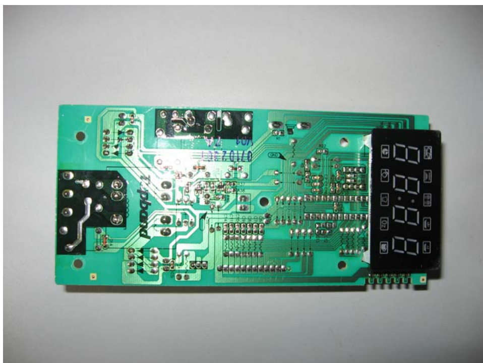
Photo 4 - Bottom view of main board
