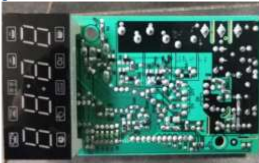
Original Mother board -bottom
