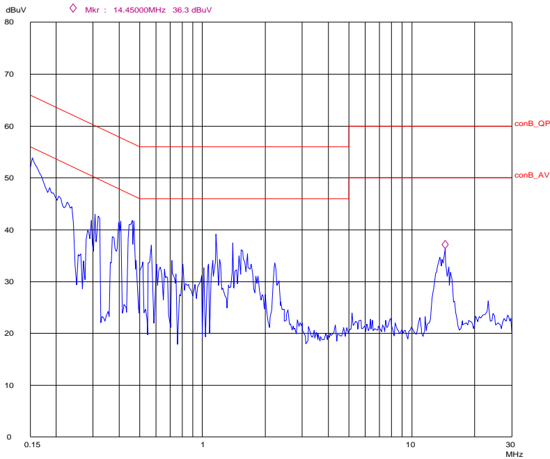
Line N Conducted Emission Graph
