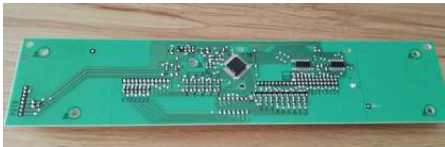
Displaying board-Bottom View
