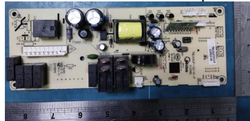
The New Mother board -top view
