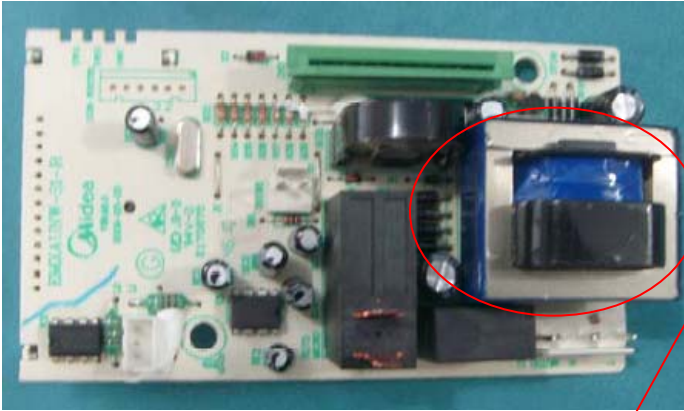
Mother board with linear transformer
