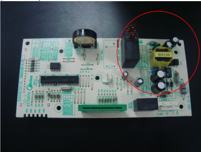
Motherboard with switching power supply (MD1001LB)
