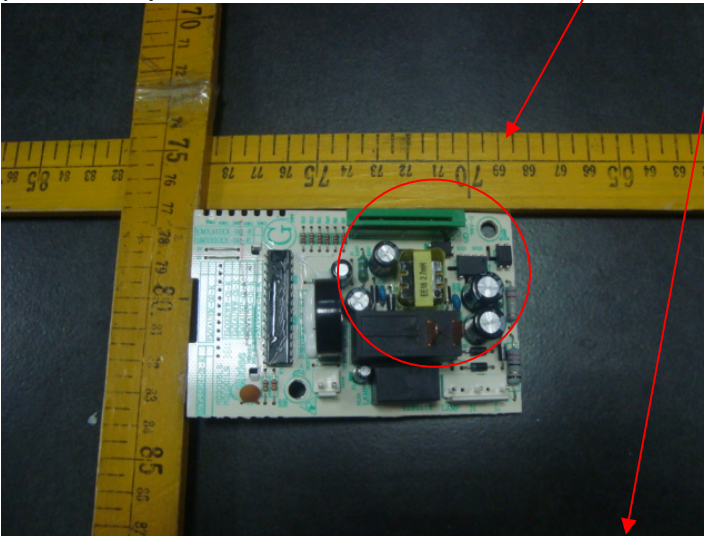
Mother board with switching power supply (MD1001LSB)
