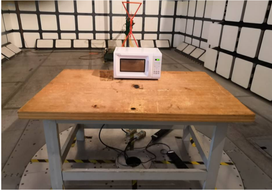
Radiated Emissions - Front View (30 MHz – 1 GHz)
