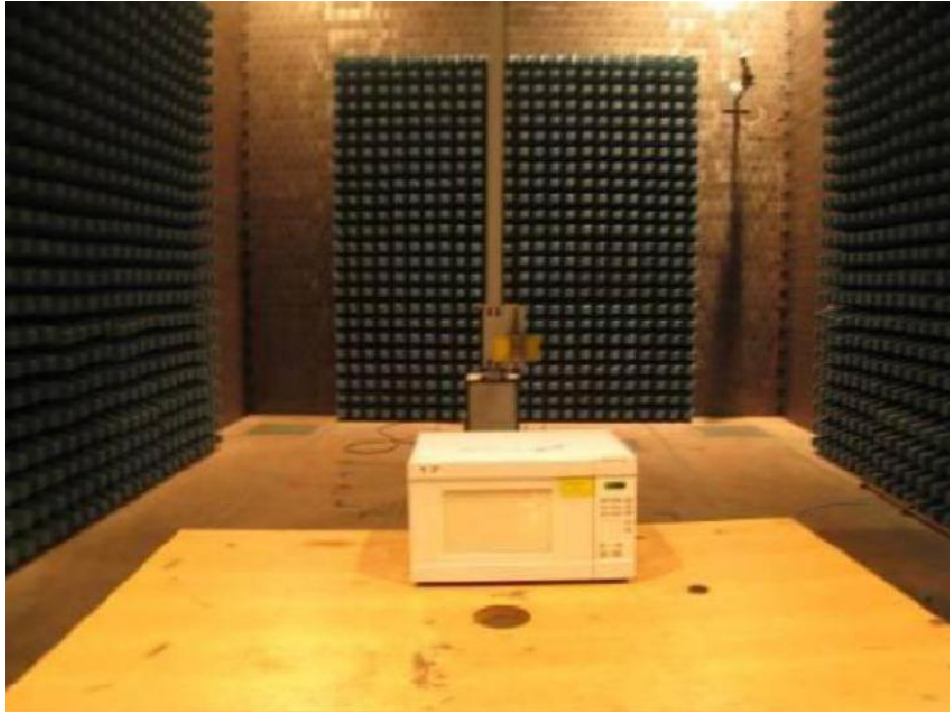
Radiated Emission
