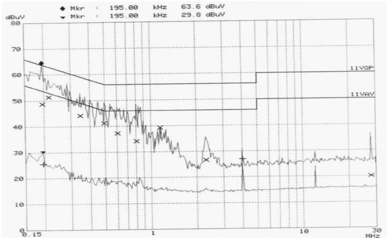
Line N Conducted Emission Graph
