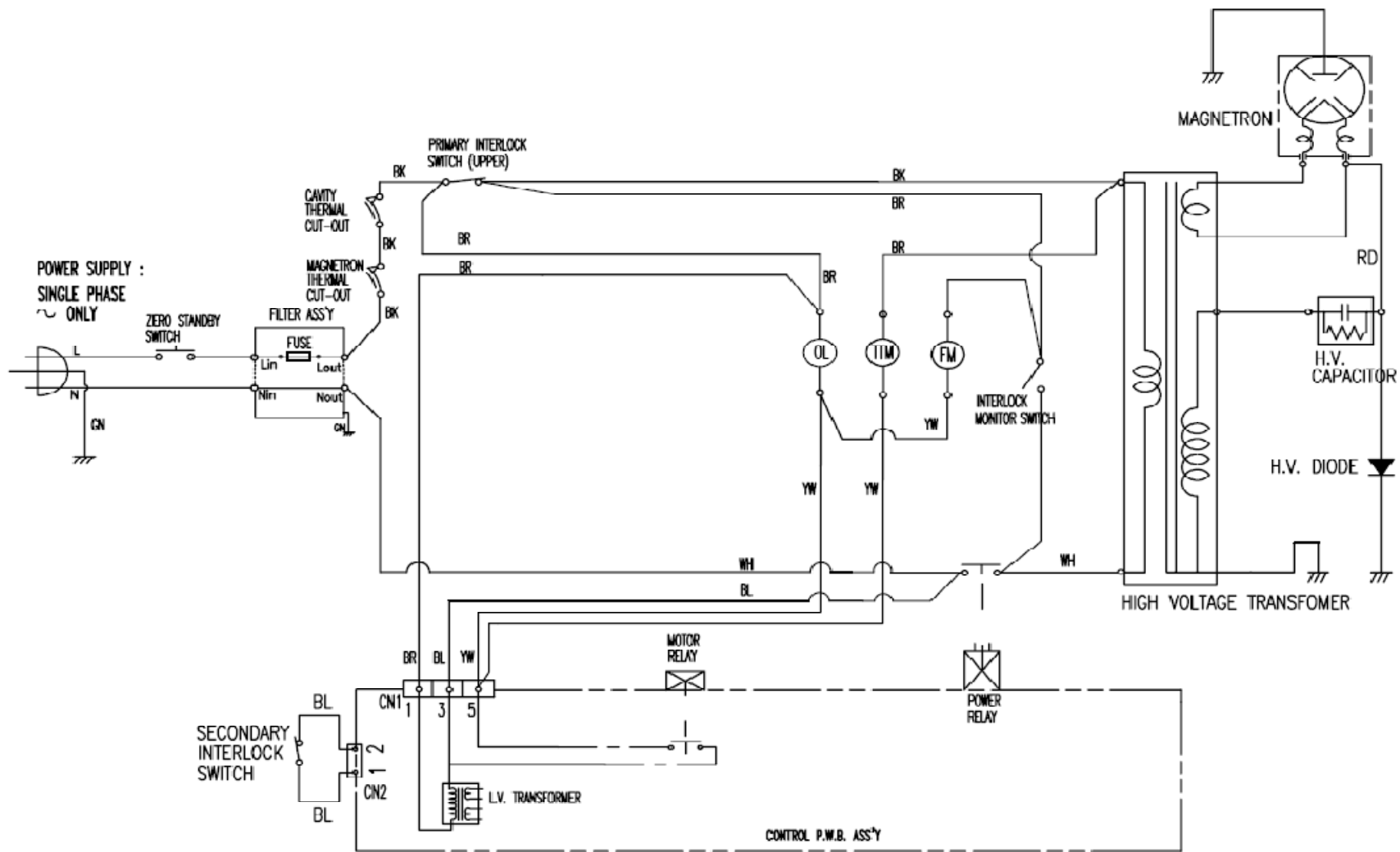
Circuit diagram
