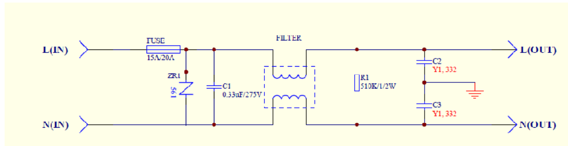
Circuit of power filter PCB
