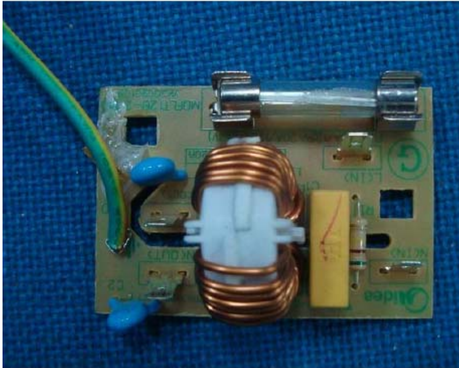
Power Filter Board -Front View
