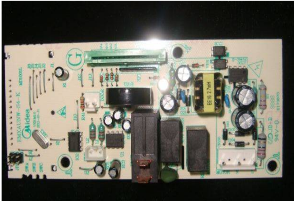
Control Board- Front View
