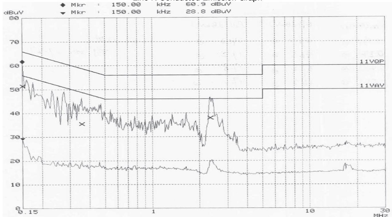
Line N Conducted Emission Graph
