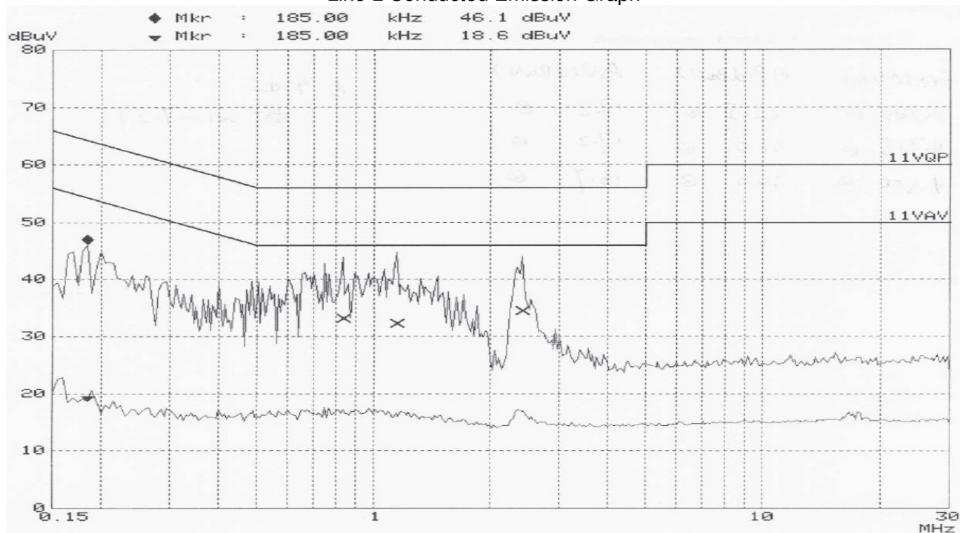
Line L Conducted Emission Graph
