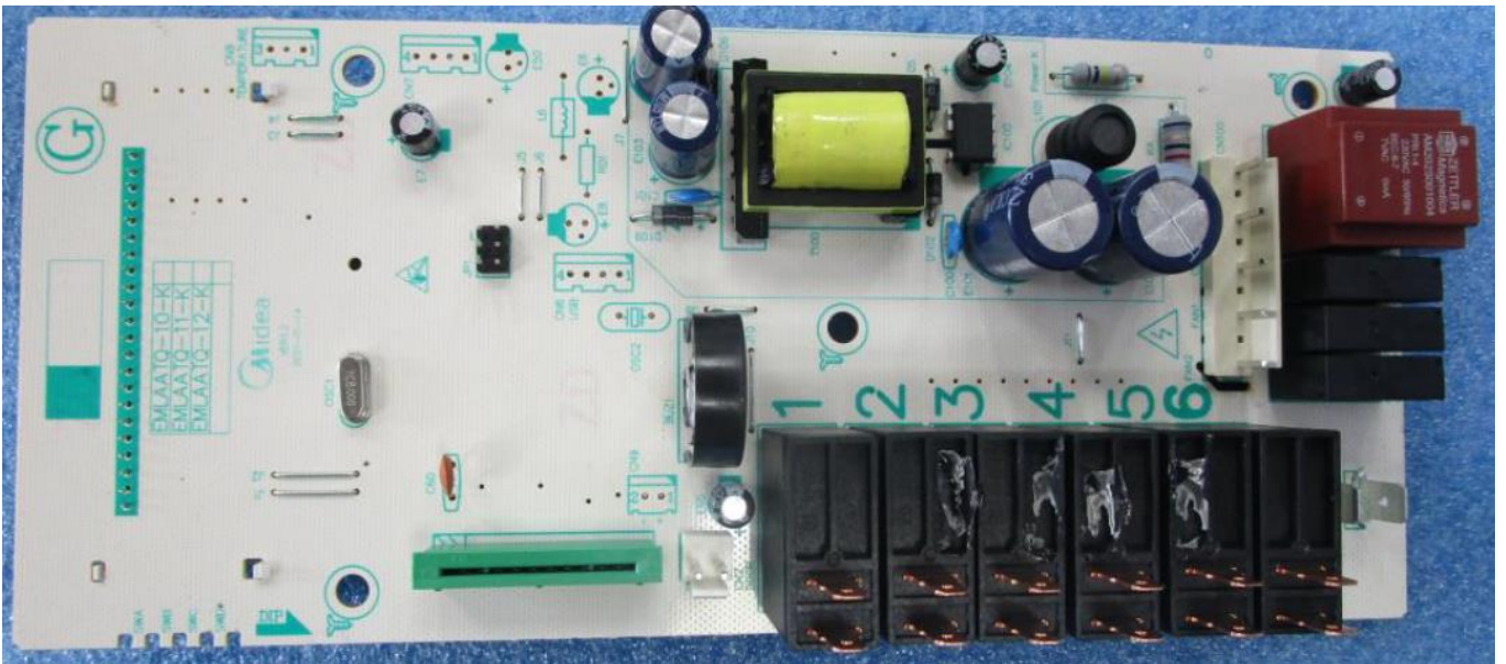
New Mother board -top view
