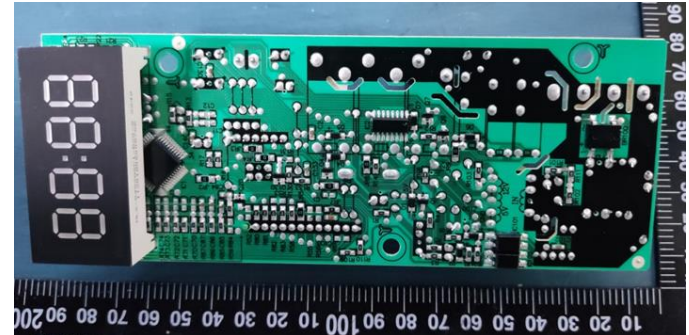
New Mother board -bottom
