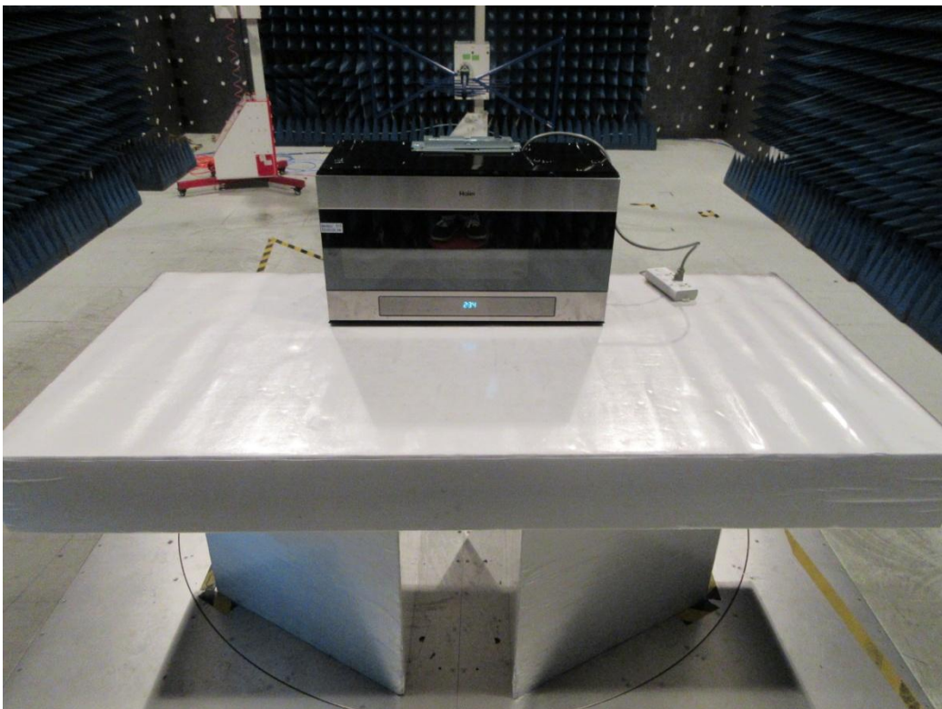
Radiated Disturbance below 1GHz
