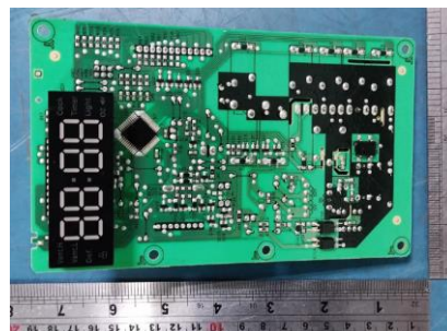
New Mother board -bottom
