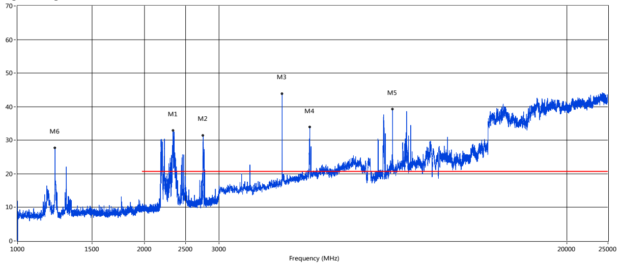
RE_EN Test Case_FCC 18 1GHz-25GHz
