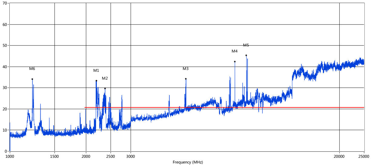
RE_EN Test Case_FCC 18 1GHz-25GHz
