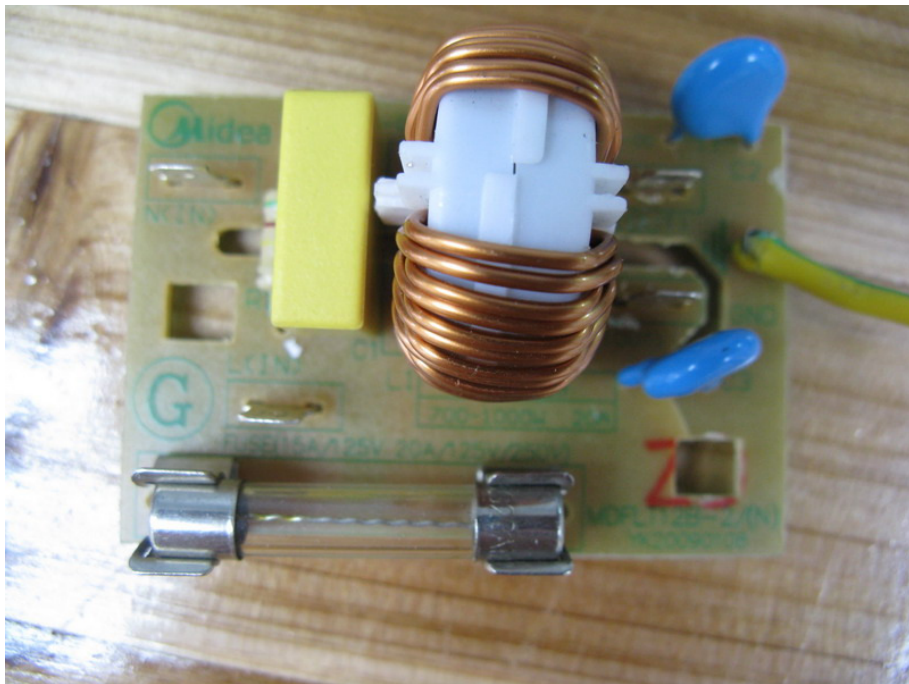
Mains filter PCB
