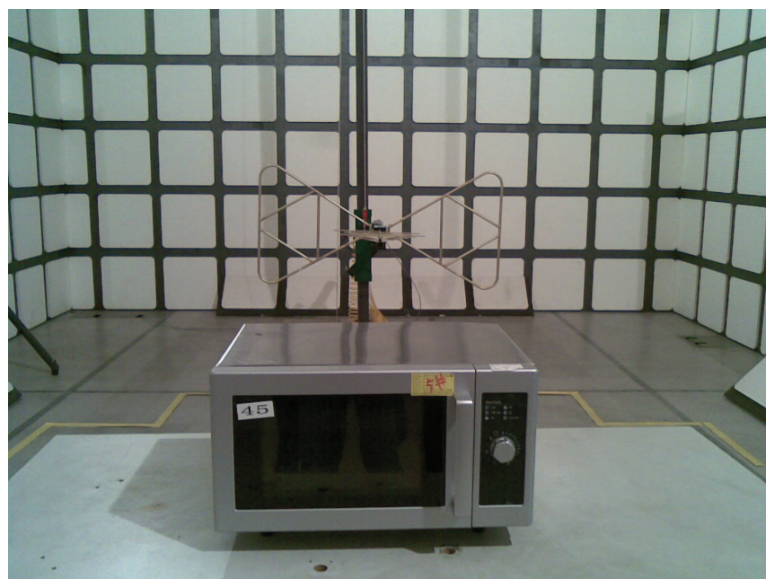
Set-up for radiation emission measurement below 1GHz
