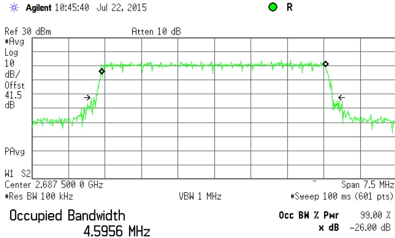
Plot 7.1.9 Occupied bandwidth test result at high frequency, 5 MHz BW, 16QAM (2687.5 MHz)
