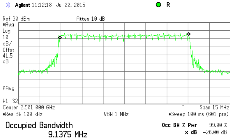
Plot 7.1.10 Occupied bandwidth test result at low frequency, 10 MHz BW, 16QAM (2501.0MHz)
