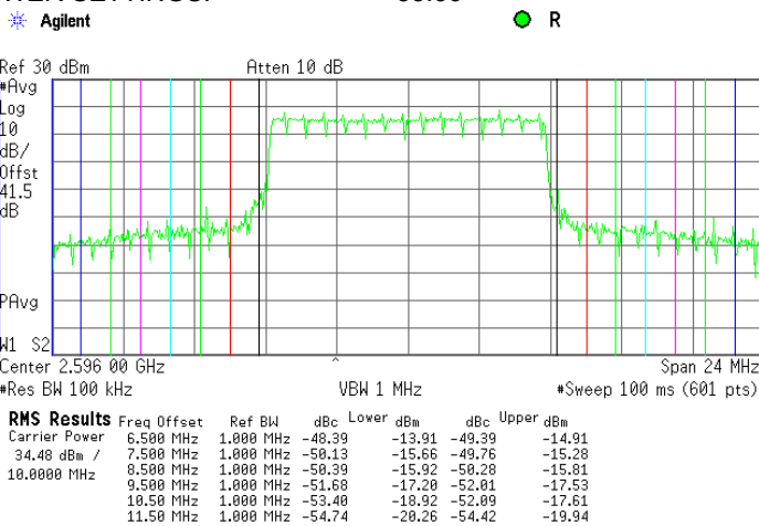
Plot 7.3.6 Spurious emission at band edges test results at high carrier frequency, 10 MHz EBW
