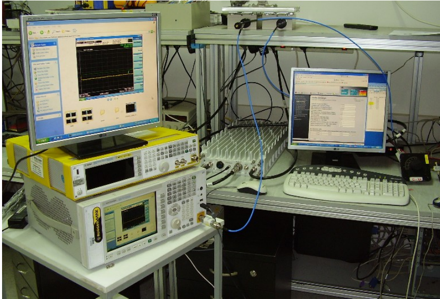
Conducted measurements. Test setup.
