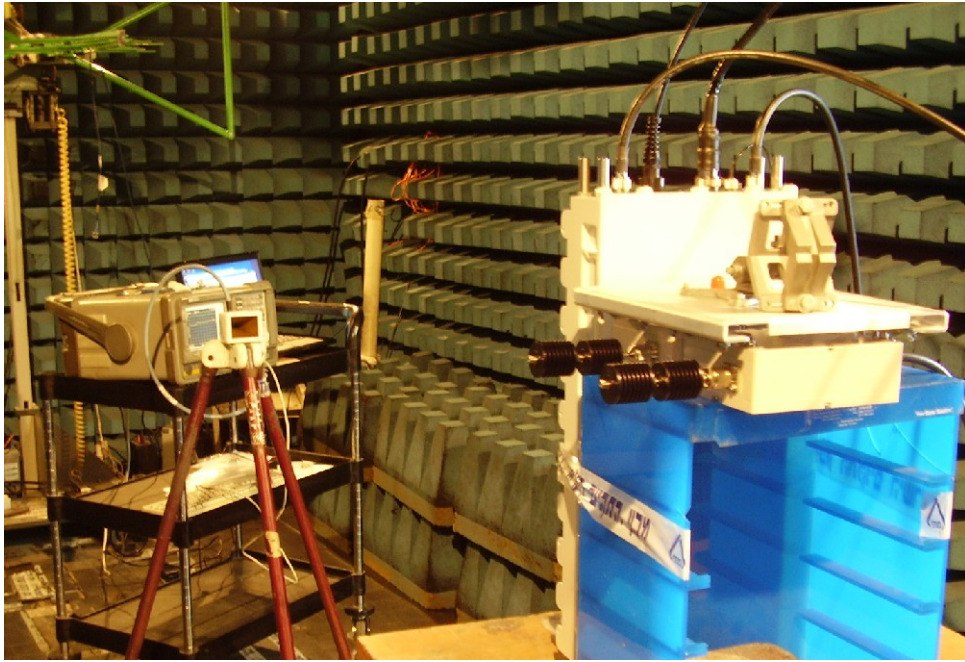
Radiated emission test setup.
