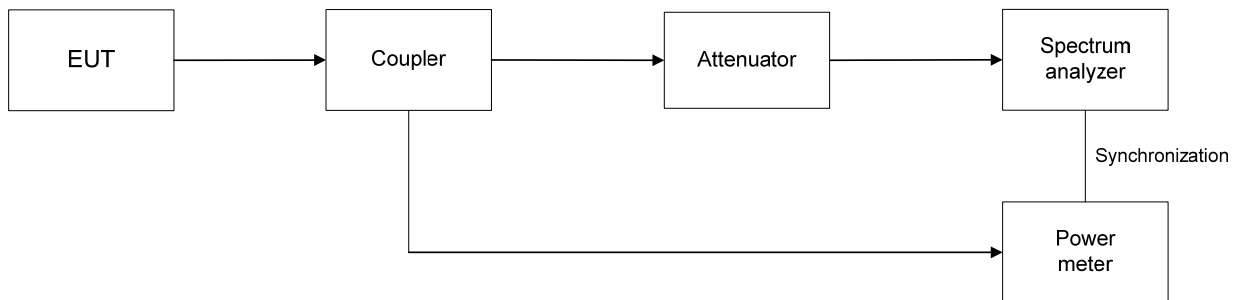
Figure 7.3.1 Setup for conducted spurious emissions
