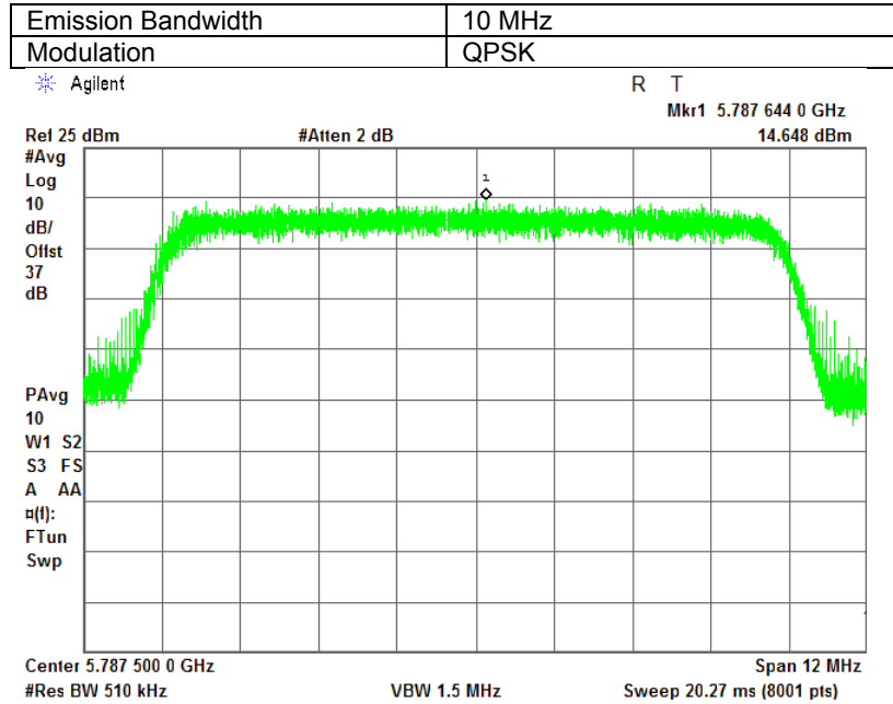
Plot 7.2.7 Peak spectral power density at mid frequency within 6 dB band, antenna gain 9.5 dBi
