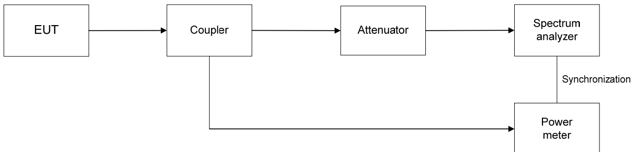
Figure 7.1.1 Peak output power test setup
