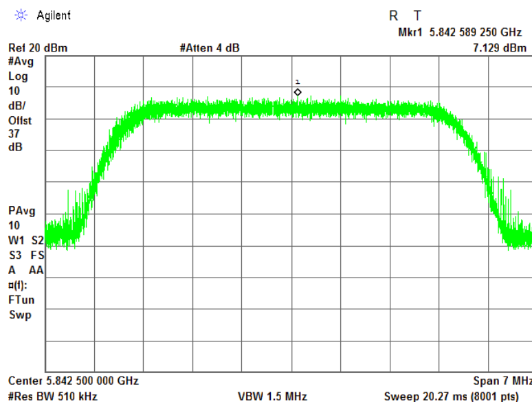
Plot 7.2.22 Peak spectral power density at high frequency within 6 dB band, antenna gain 22.5 dBi
