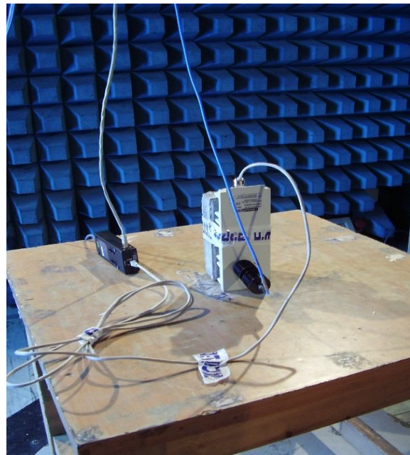
Radiated emission test setup. General EUT view.
