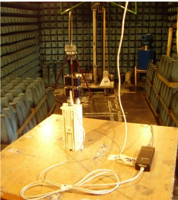
Radiated emission test setup.
