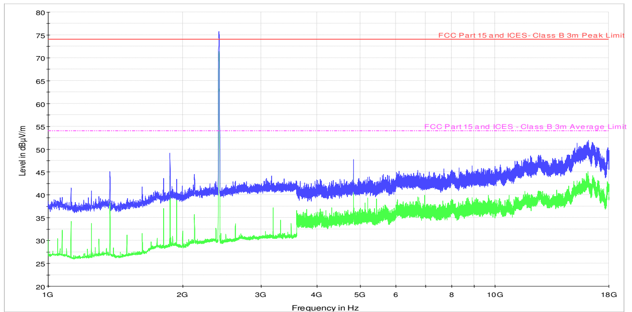
Figure 8.4-27: Radiated spurious emissions for 802.11b, sample plot
