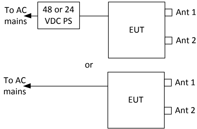
Figure 3.6-1: Setup diagram
