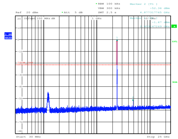
Figure 8.4-14: Conducted spurious emissions for MIMO, low channel, ch1
