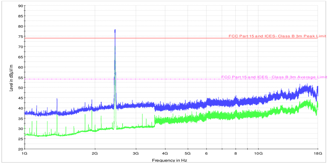
Figure 8.4-28: Radiated spurious emissions for 802.11g, sample plot
