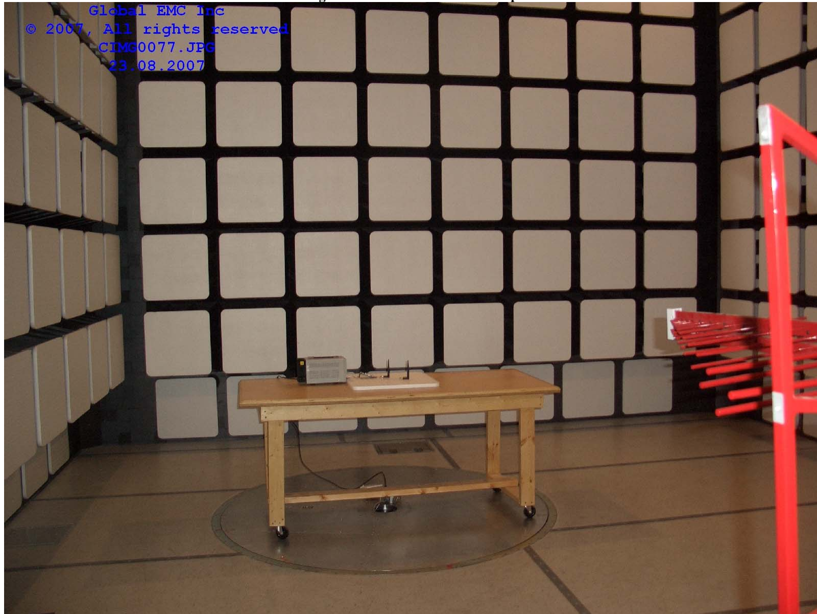
Figure 1 - Radiated Emissions Setup
