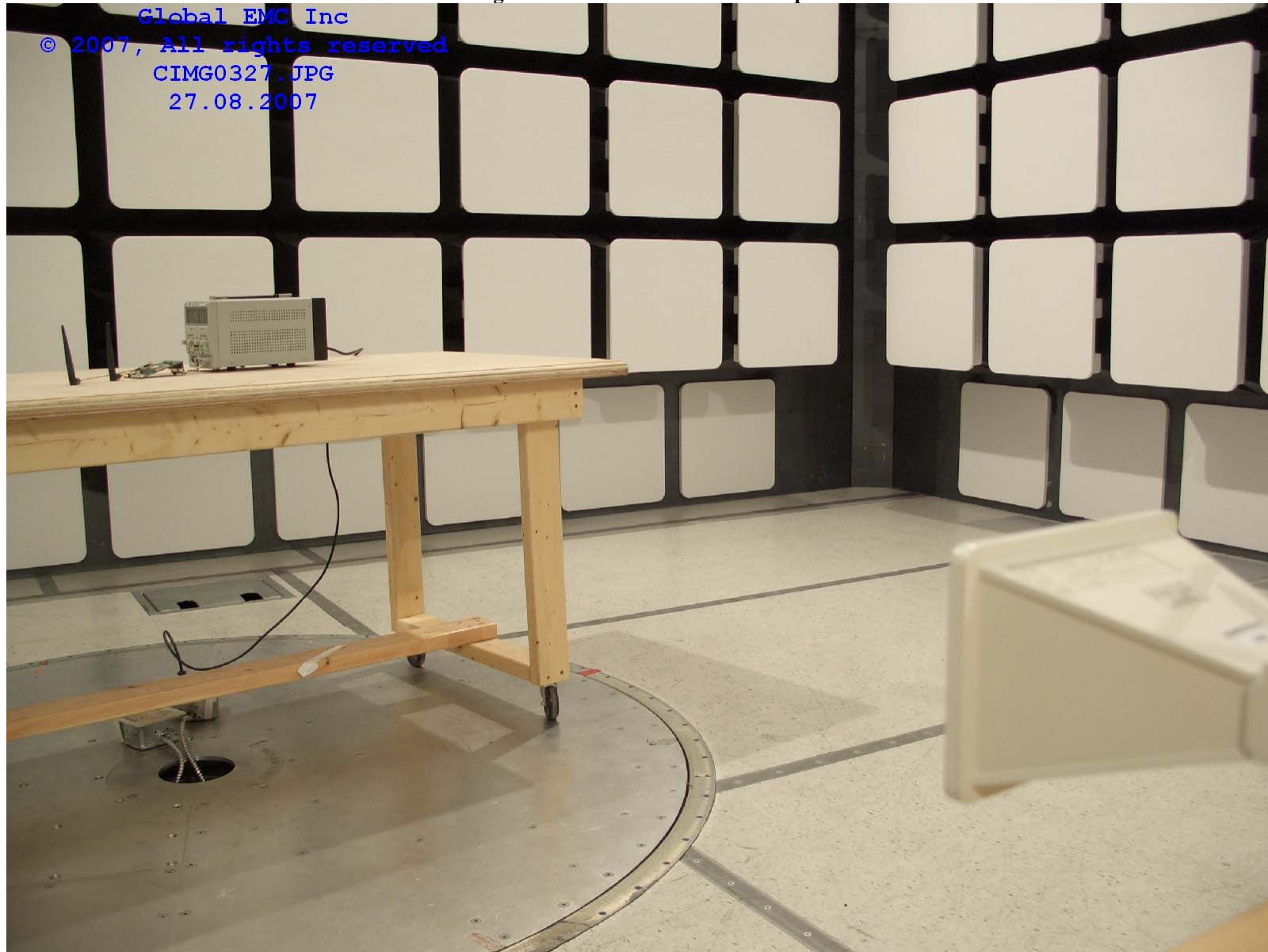
Figure 3 – Radiated Emissions Setup
