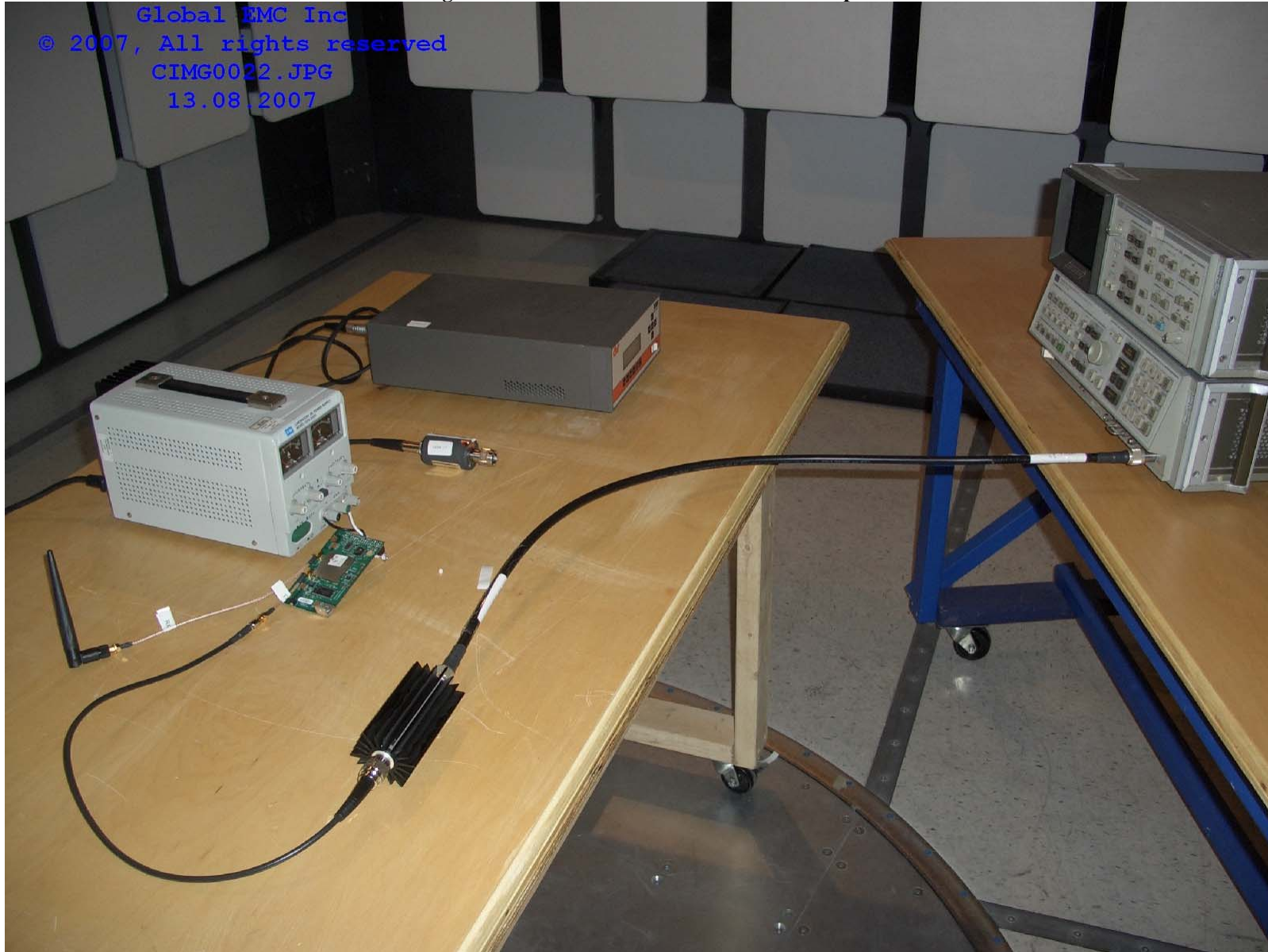
Figure 5 – Antenna Conducted Emissions Setup
