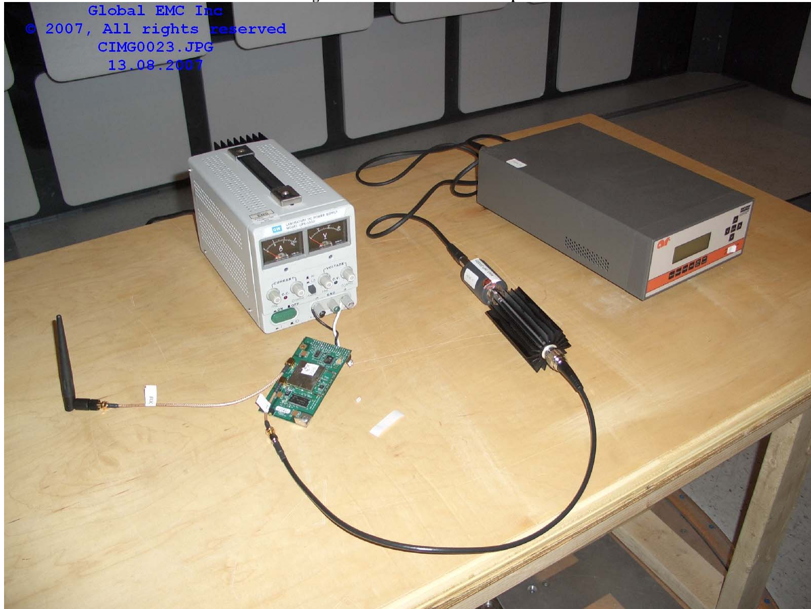
Figure 4 – Power Measurement Setup
