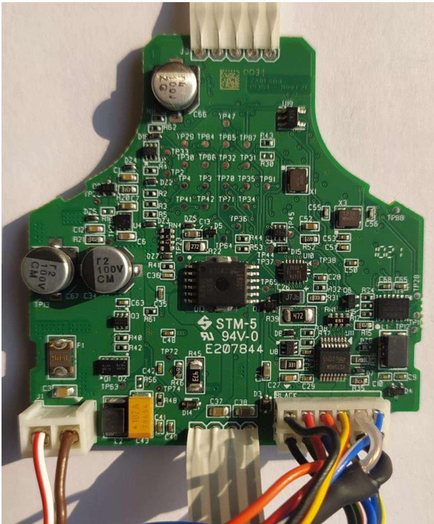
Figure 2 – Main board Top side
