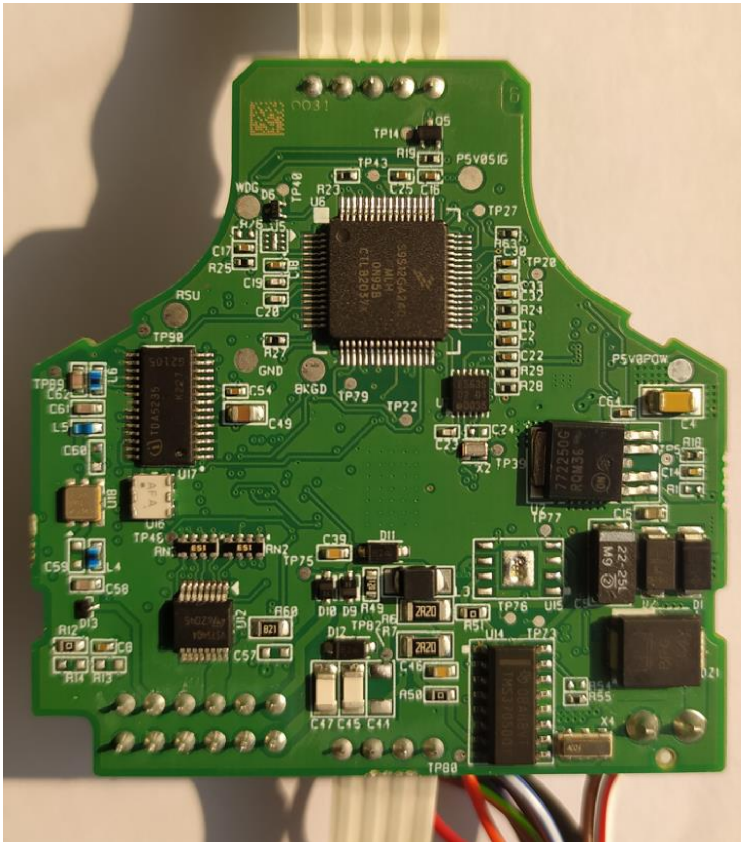
Figure 1 – Main board bottom side
