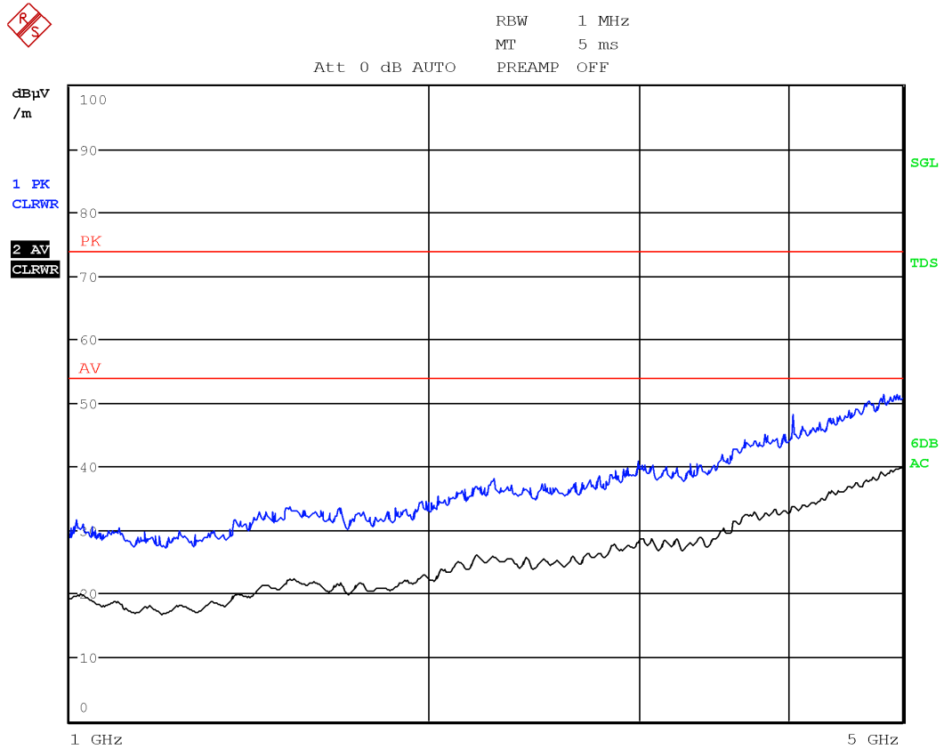
Antenna in horizontal polarization @ 3 m
