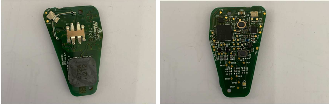
Figure 3.5-1: EUT overview
