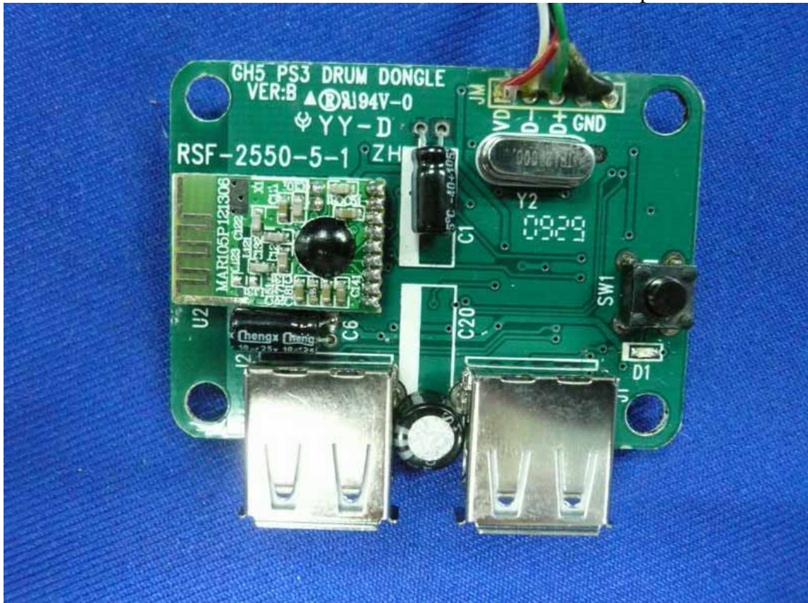
Figure 1 Components Side of the PCB
