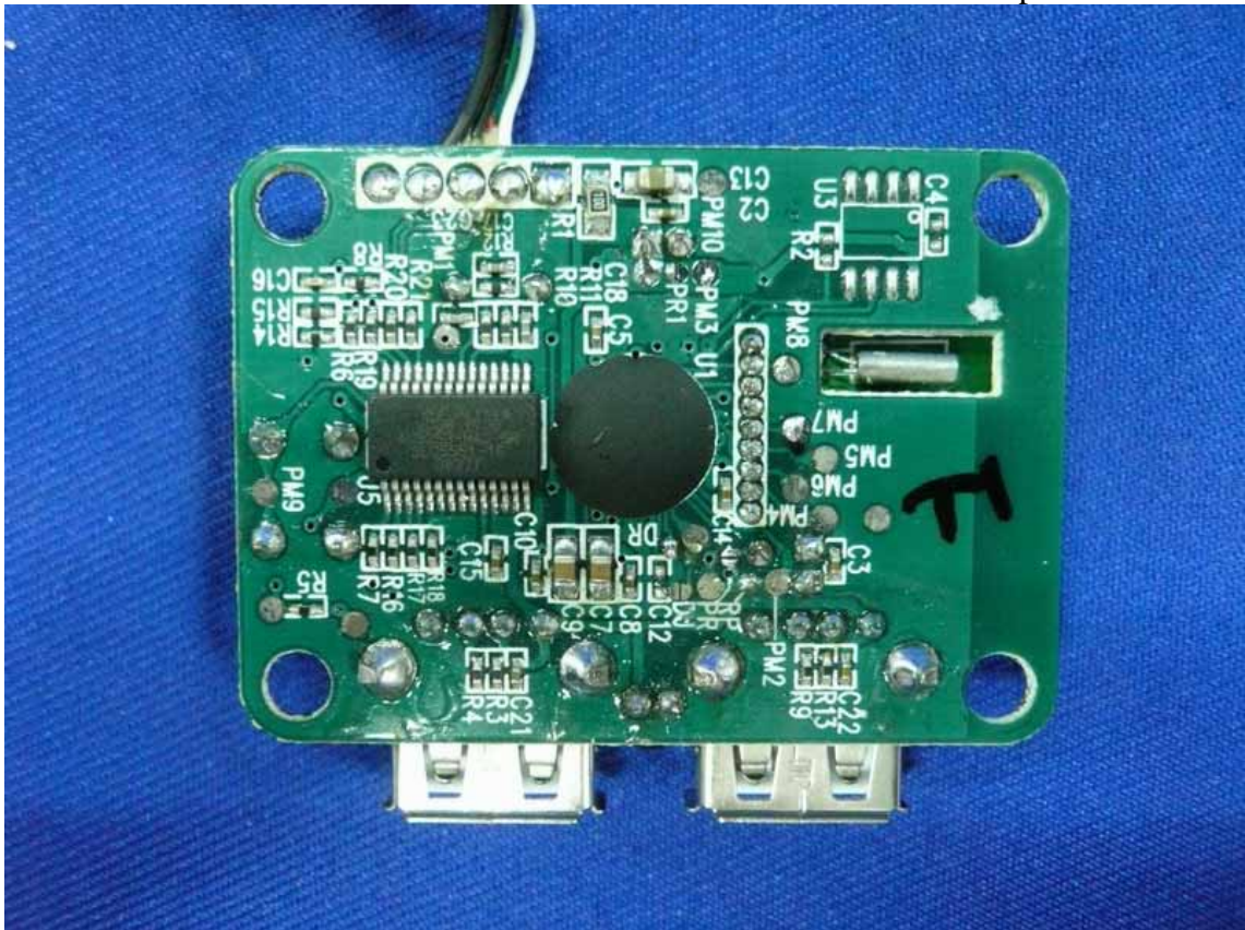
Figure 3 Components Side of the PCB
