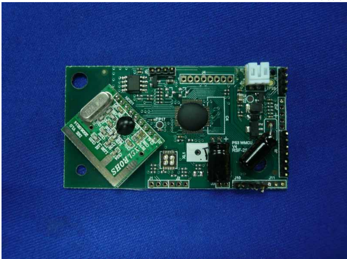
Figure 41 Inside of the EUT
