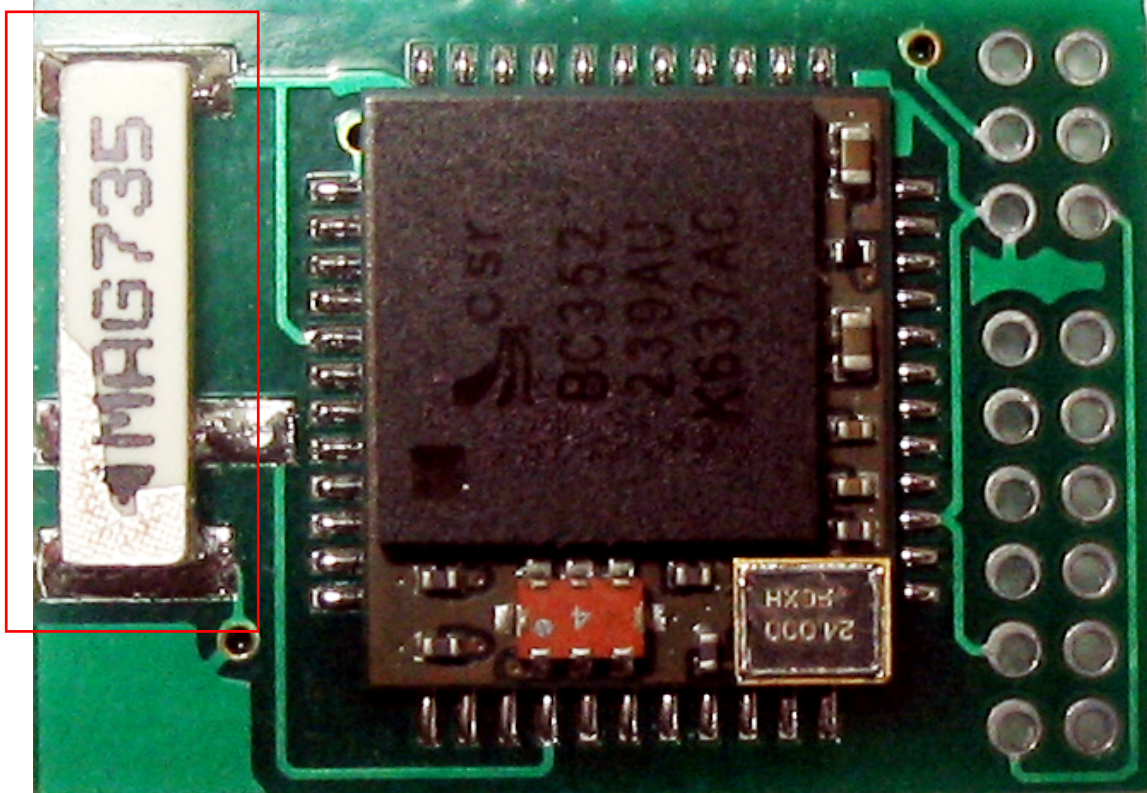
Chip Antenna
