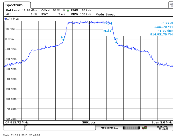
Figure 7.2.2-23: 20 dB OBW - Middle Channel (QPSK, Antenna Path 2)
