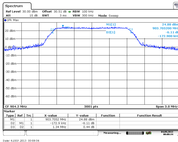
Figure 7.2.2-13: 6dB BW - Low Channel (QPSK, Antenna Path 1)
