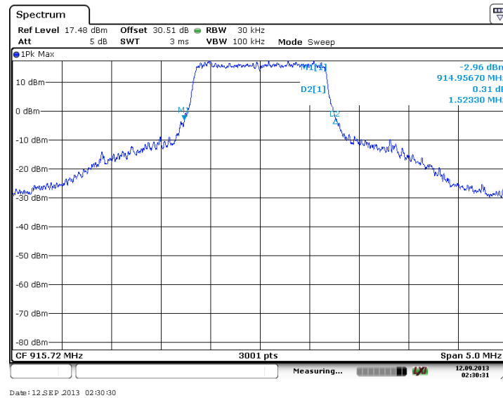
Figure 7.2.2-41: 20 dB OBW - Middle Channel (64-QAM, Antenna Path 1)
