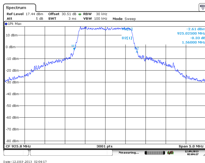
Figure 7.2.2-18: 20 dB OBW - High Channel (QPSK, Antenna Path 1)
