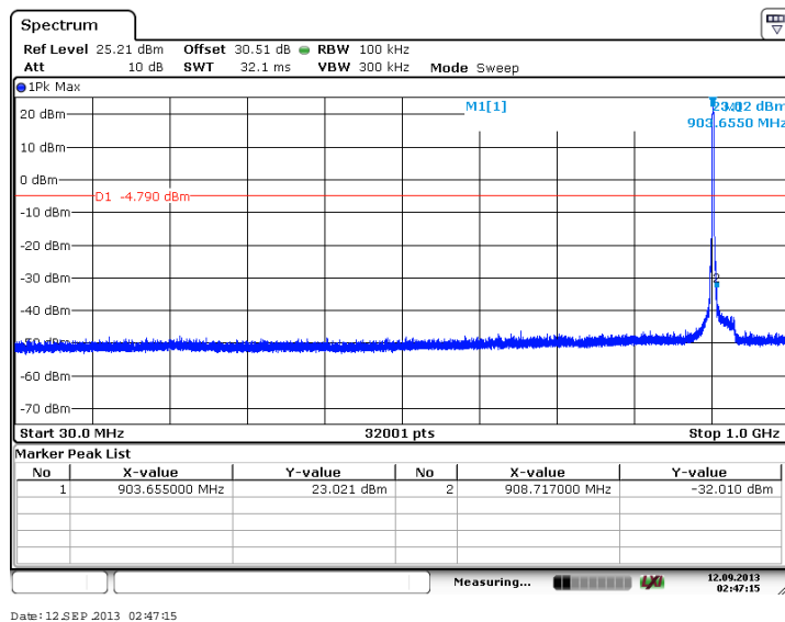
Figure 7.4.2.2-37: 30 MHz – 1 GHz – Low Channel (64-QAM, Antenna Path 1)
