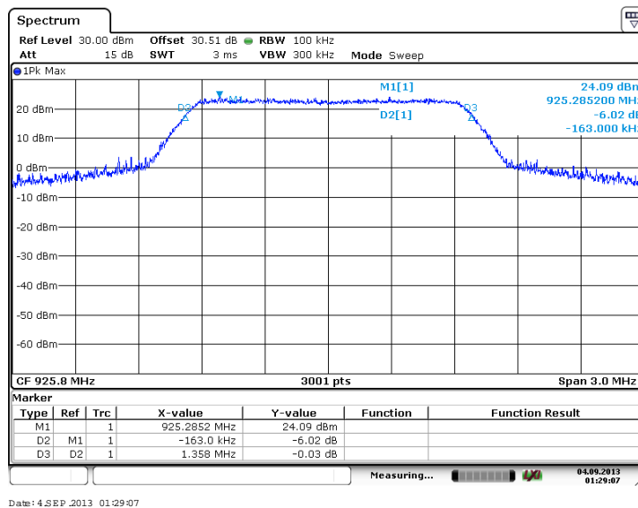
Figure 7.2.2-27: 6dB BW - High Channel (16-QAM, Antenna Path 1)
