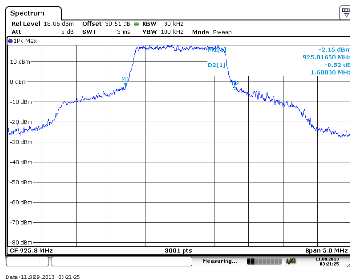
Figure 7.2.2-12: 20 dB OBW - High Channel (BPSK, Antenna Path 2)
