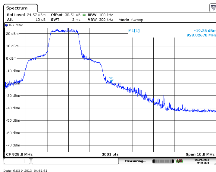
Figure 7.4.1.2-16: Upper Band-edge (64-QAM, Antenna Path 2)
