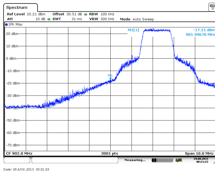
Figure 7.4.1.2-13: Lower Band-edge (64-QAM, Antenna Path 1)
