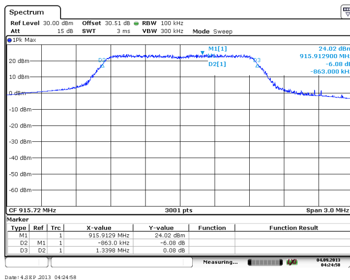
Figure 7.2.2-8: 6dB BW - Middle Channel (BPSK, Antenna Path 2)
