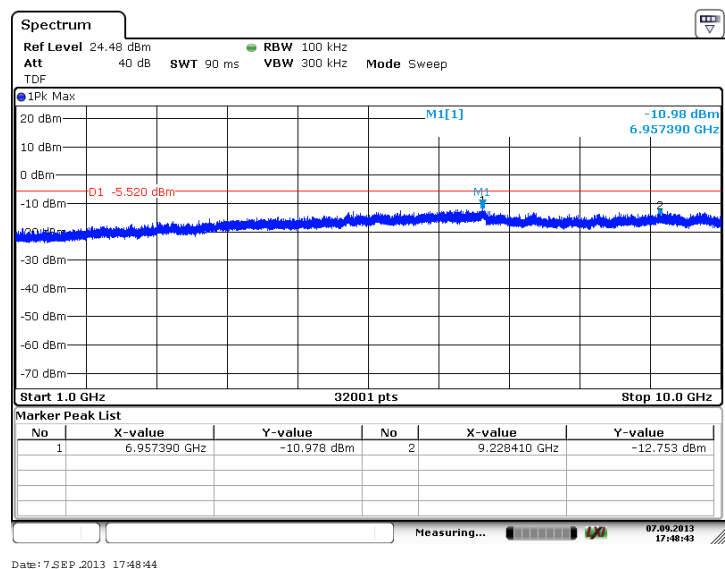
Figure 7.4.2.2-8: 1 GHz – 10 GHz – Low Channel (BPSK, Antenna Path 2)
