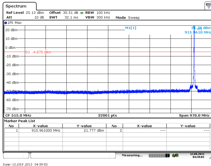
Figure 7.4.2.2-45: 30 MHz – 1 GHz – Middle Channel (64-QAM, Antenna Path 2)
