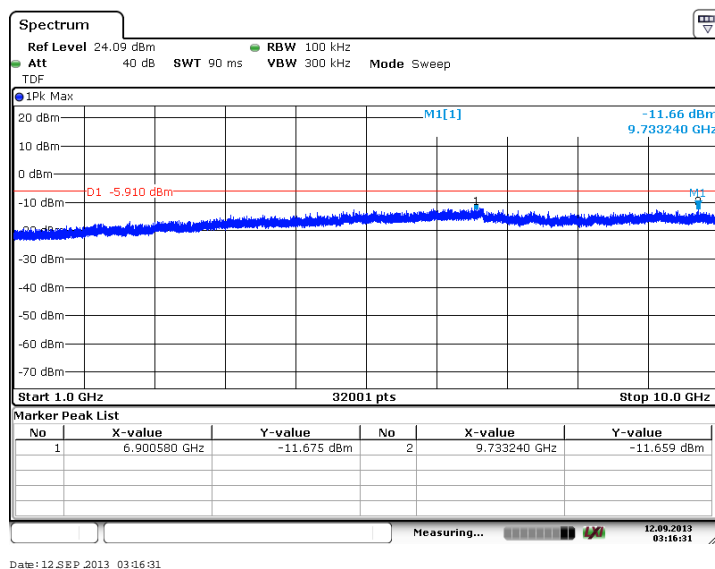
Figure 7.4.2.2-30: 1 GHz – 10 GHz – High Channel (16-QAM, Antenna Path 1)
