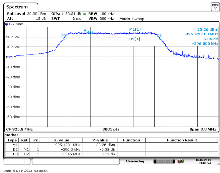
Figure 7.2.2-9: 6dB BW - High Channel (BPSK, Antenna Path 2)
