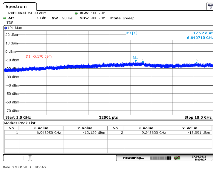
Figure 7.4.2.2-6: 1 GHz – 10 GHz – High Channel (BPSK, Antenna Path 1)
