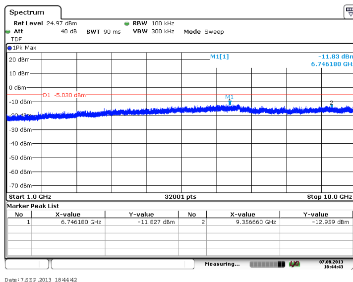
Figure 7.4.2.2-44: 1 GHz – 10 GHz – Low Channel (64-QAM, Antenna Path 2)
