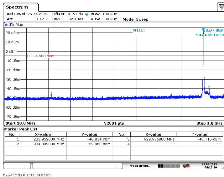
Figure 7.4.2.2-31: 30 MHz – 1 GHz – Low Channel (16-QAM, Antenna Path 2)
