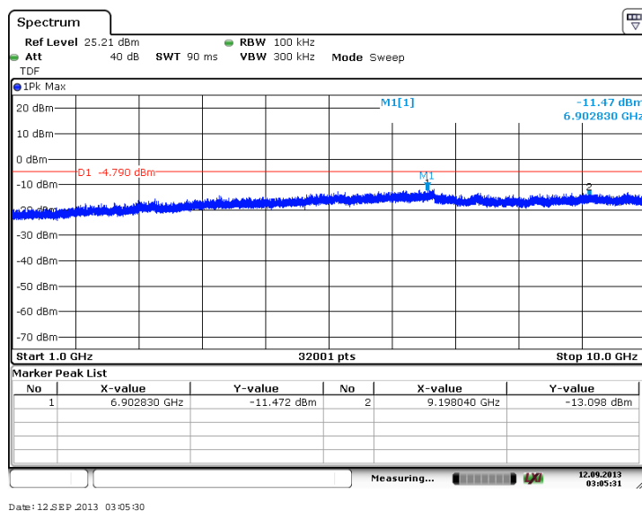
Figure 7.4.2.2-38: 1 GHz – 10 GHz – Low Channel (64-QAM, Antenna Path 1)
