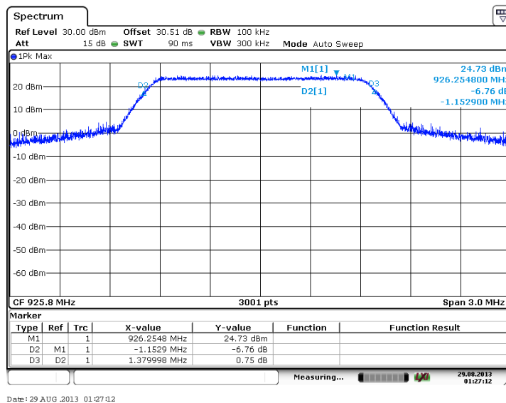
Figure 7.2.2-39: 6dB BW - High Channel (64-QAM, Antenna Path 1)
