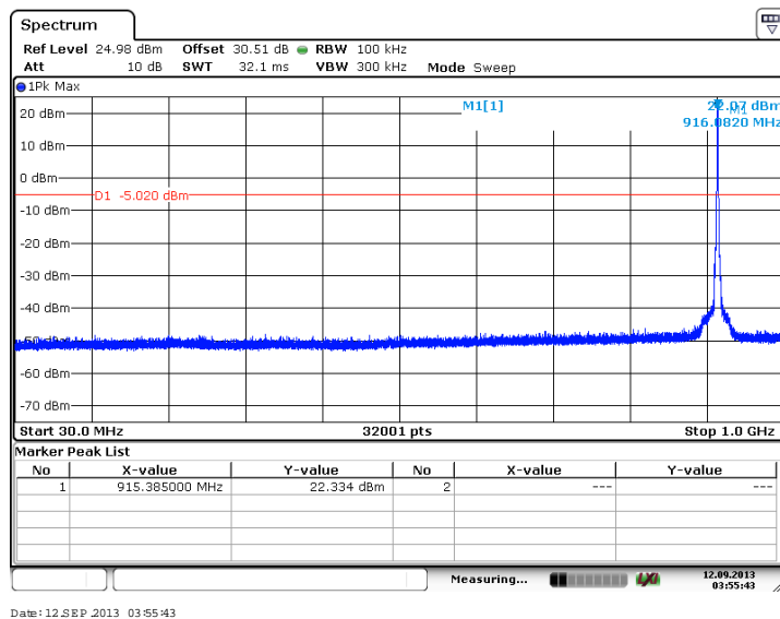
Figure 7.4.2.2-15: 30 MHz – 1 GHz – Middle Channel (QPSK, Antenna Path 1)
