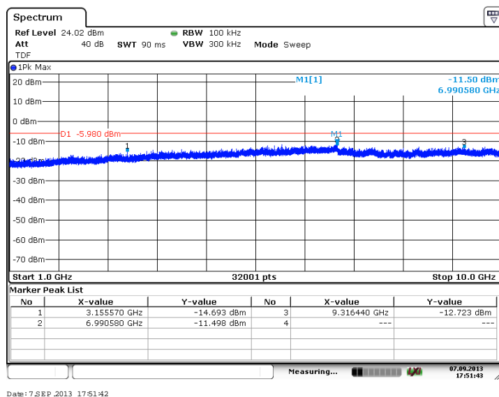
Figure 7.4.2.2-10: 1 GHz – 10 GHz – Middle Channel (BPSK, Antenna Path 2)
