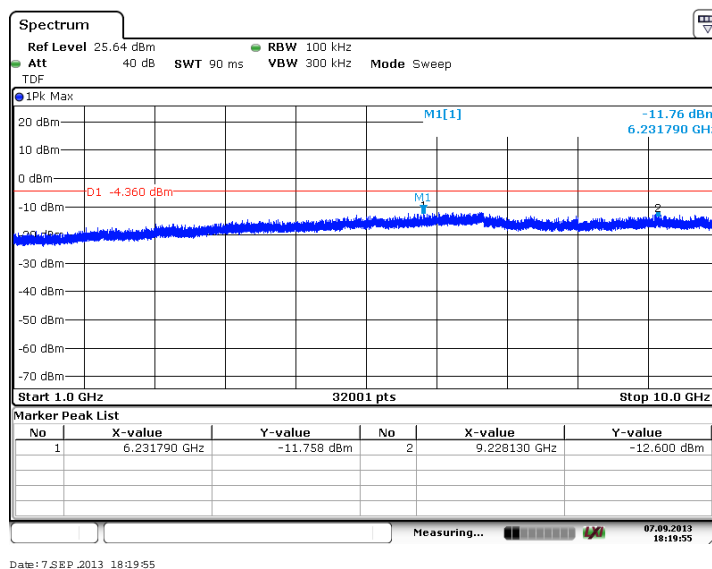
Figure 7.4.2.2-36: 1 GHz – 10 GHz – High Channel (16-QAM, Antenna Path 2)
