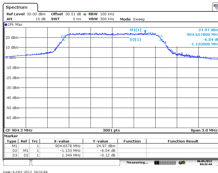
Figure 7.2.2-43: 6dB BW - Low Channel (64-QAM, Antenna Path 2)
