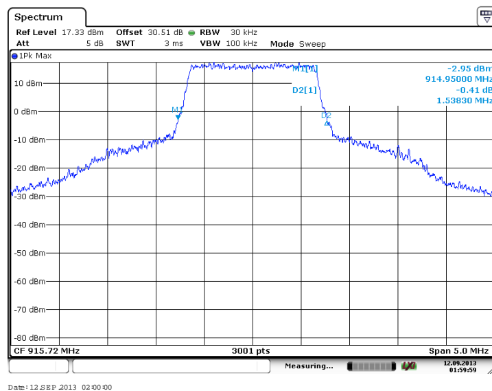
Figure 7.2.2-17: 20 dB OBW - Middle Channel (QPSK, Antenna Path 1)
