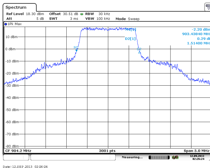
Figure 7.2.2-40: 20 dB OBW - Low Channel (64-QAM, Antenna Path 1)
