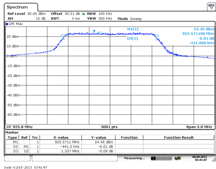
Figure 7.2.2-21: 6dB BW - High Channel (QPSK, Antenna Path 2)
