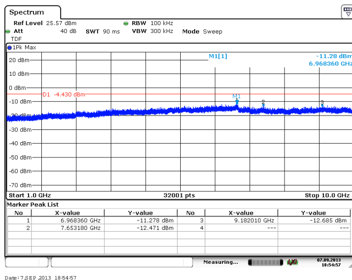
Figure 7.4.2.2-4: 1 GHz – 10 GHz – Middle Channel (BPSK, Antenna Path 1)
