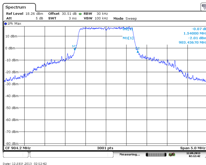
Figure 7.2.2-28: 20 dB OBW - Low Channel (16-QAM, Antenna Path 1)
