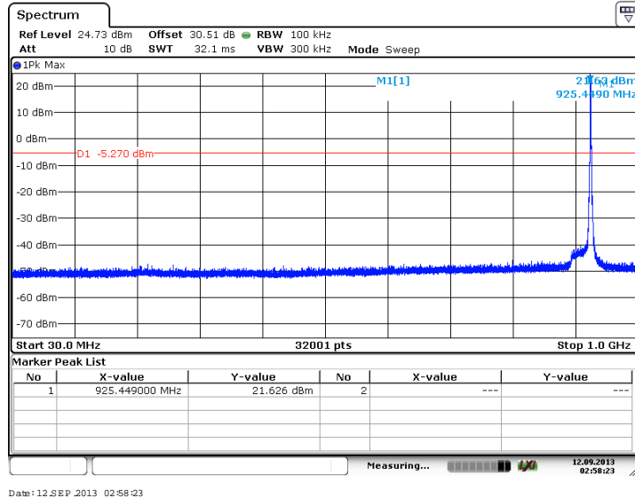
Figure 7.4.2.2-41: 30 MHz – 1 GHz – High Channel (64-QAM, Antenna Path 1)
