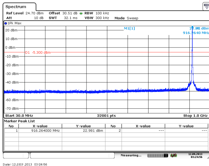
Figure 7.4.2.2-27: 30 MHz – 1 GHz – Middle Channel (16-QAM, Antenna Path 1)
