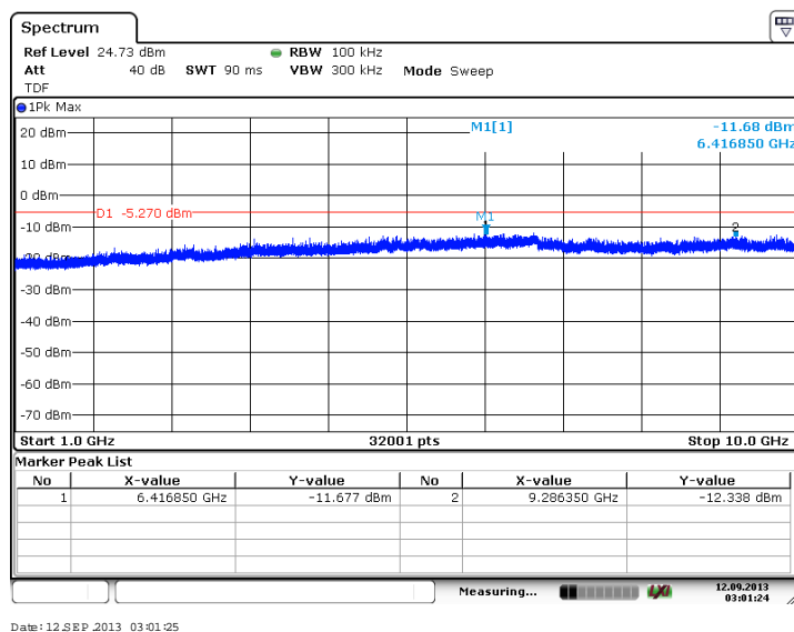
Figure 7.4.2.2-42: 1 GHz – 10 GHz – High Channel (64-QAM, Antenna Path 1)
