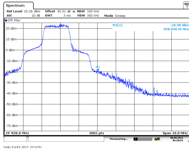
Figure 7.4.1.2-4: Upper Band-edge (BPSK, Antenna Path 2)
