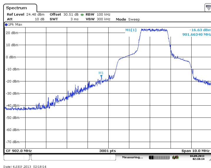
Figure 7.4.1.2-3: Lower Band-edge (BPSK, Antenna Path 2)
