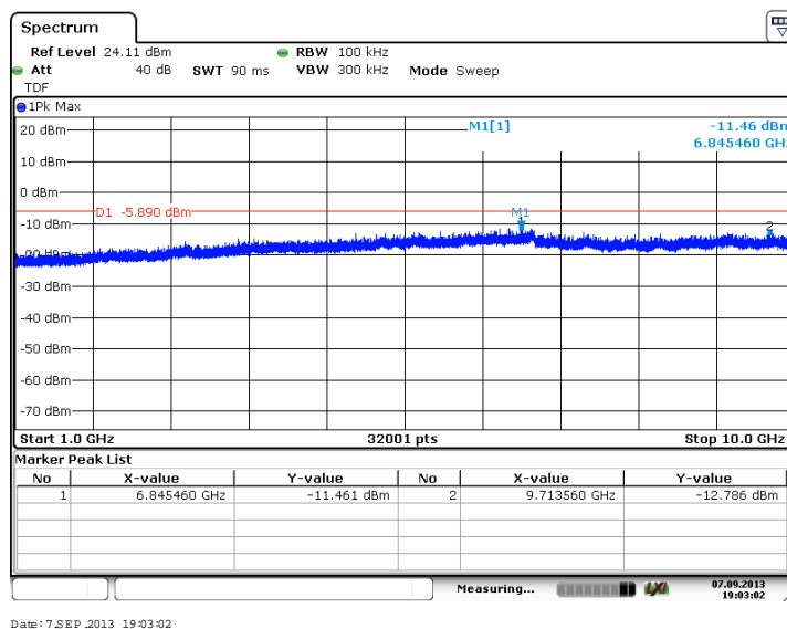
Figure 7.4.2.2-18: 1 GHz – 10 GHz – High Channel (QPSK, Antenna Path 1)
