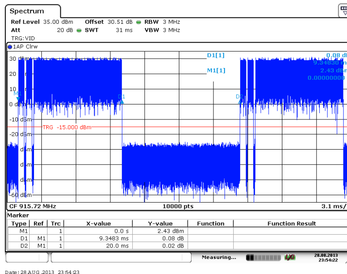
Figure 7.6.2-1: Duty Cycle
