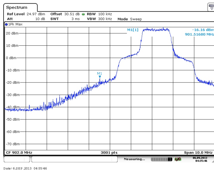
Figure 7.4.1.2-15: Lower Band-edge (64-QAM, Antenna Path 2)
