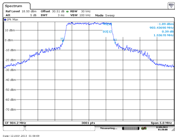
Figure 7.2.2-4: 20 dB OBW - Low Channel (BPSK, Antenna Path 1)
