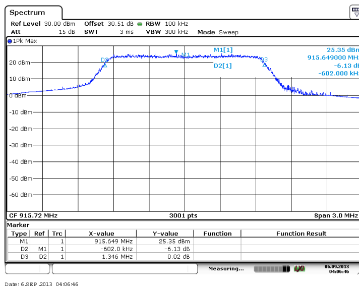
Figure 7.2.2-32: 6dB BW - Middle Channel (16-QAM, Antenna Path 2)
