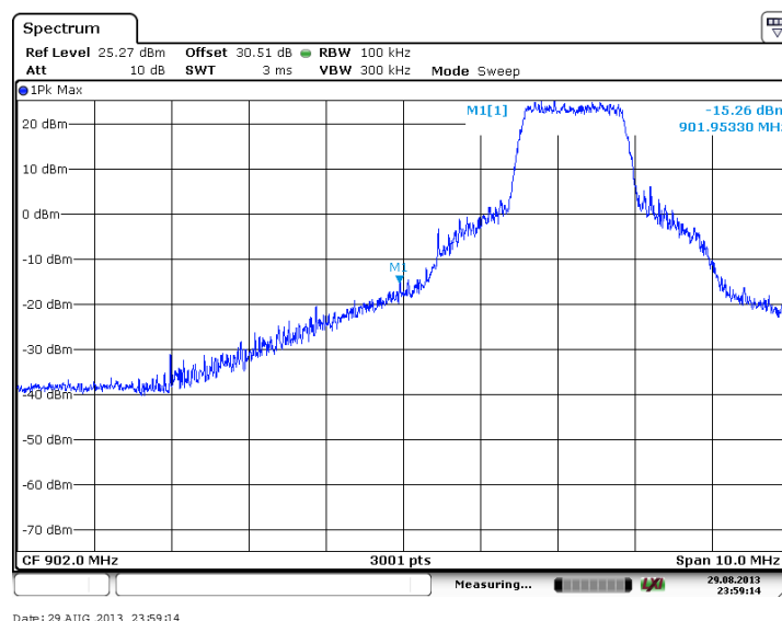
Figure 7.4.1.2-1: Lower Band-edge (BPSK, Antenna Path 1)
