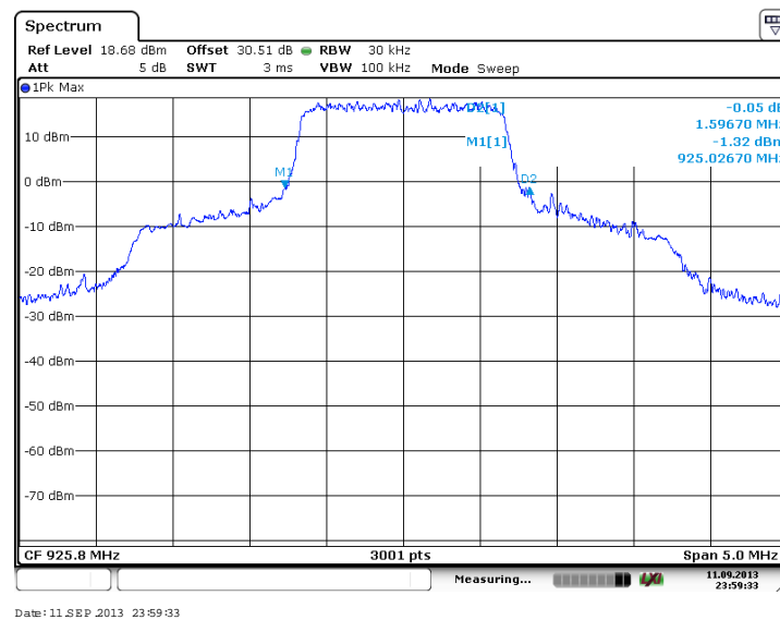
Figure 7.2.2-24: 20 dB OBW - High Channel (QPSK, Antenna Path 2)
