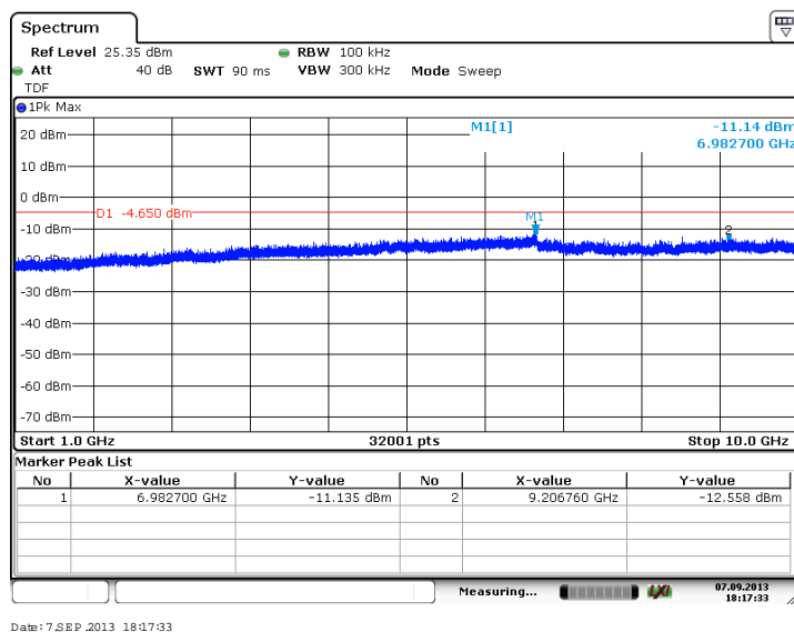
Figure 7.4.2.2-34: 1 GHz – 10 GHz – Middle Channel (16-QAM, Antenna Path 2)
