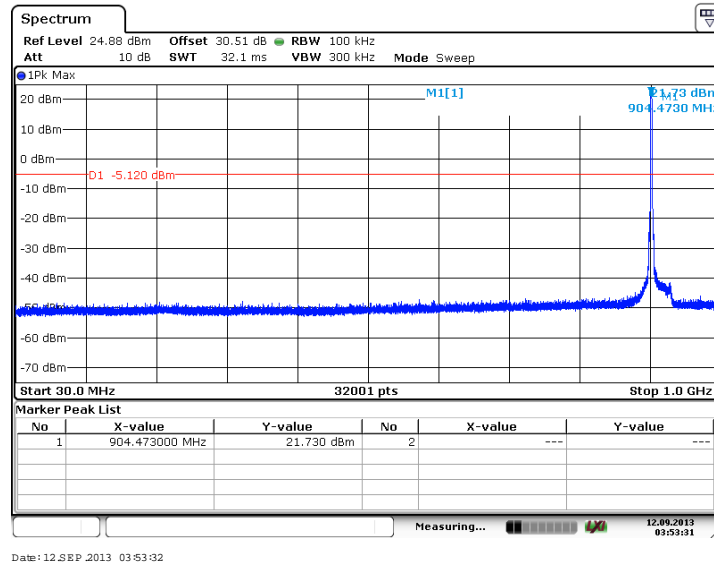
Figure 7.4.2.2-13: 30 MHz – 1 GHz – Low Channel (QPSK, Antenna Path 1)
