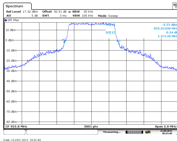
Figure 7.2.2-30: 20 dB OBW - High Channel (16-QAM, Antenna Path 1)
