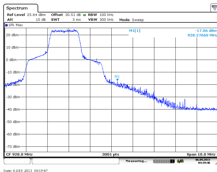
Figure 7.4.1.2-12: Upper Band-edge (16-QAM, Antenna Path 2)
