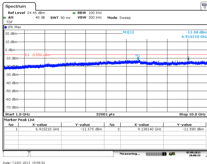
Figure 7.4.2.2-24: 1 GHz – 10 GHz – High Channel (QPSK, Antenna Path 2)
