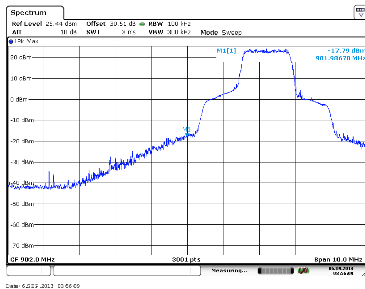
Figure 7.4.1.2-11: Lower Band-edge (16-QAM, Antenna Path 2)
