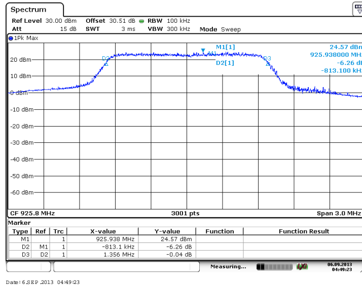
Figure 7.2.2-45: 6dB BW - High Channel (64-QAM, Antenna Path 2)
