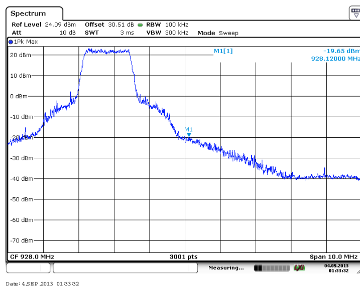
Figure 7.4.1.2-10: Upper Band-edge (16-QAM, Antenna Path 1)
