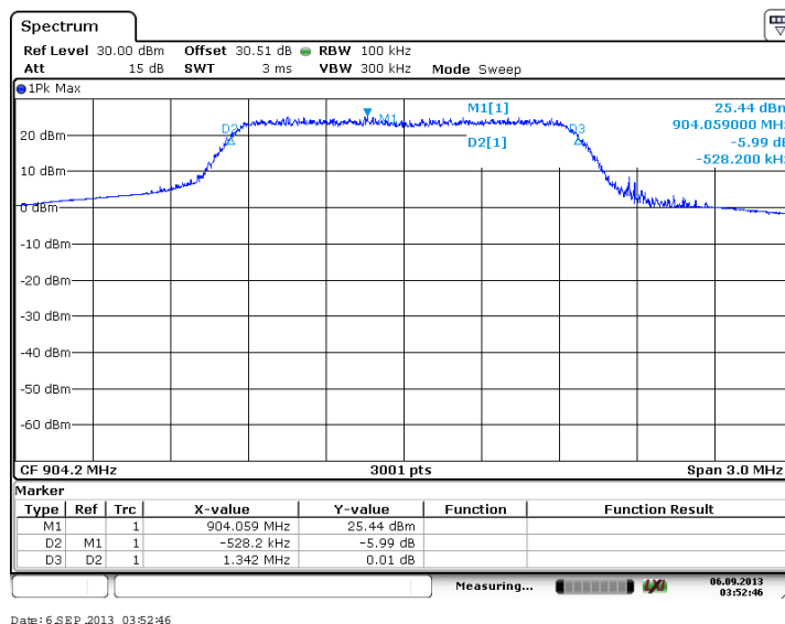
Figure 7.2.2-31: 6dB BW - Low Channel (16-QAM, Antenna Path 2)
