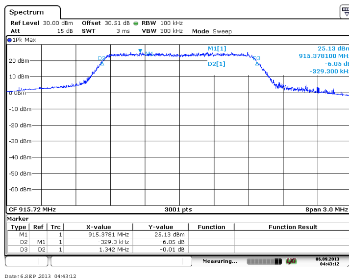
Figure 7.2.2-44: 6dB BW - Middle Channel (64-QAM, Antenna Path 2)
