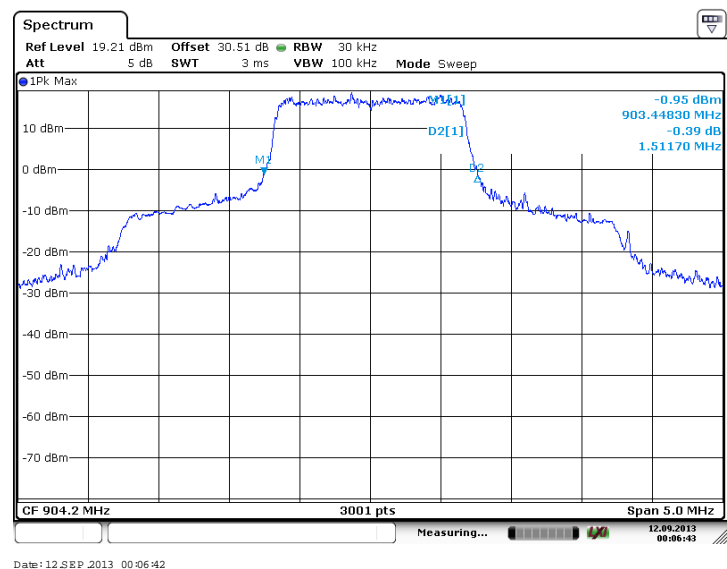
Figure 7.2.2-34: 20 dB OBW - Low Channel (16-QAM, Antenna Path 2)
