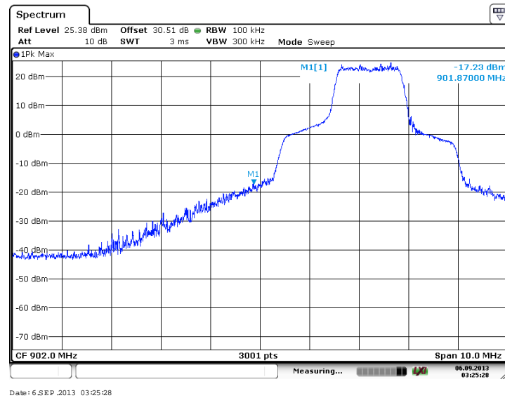
Figure 7.4.1.2-7: Lower Band-edge (QPSK, Antenna Path 2)
