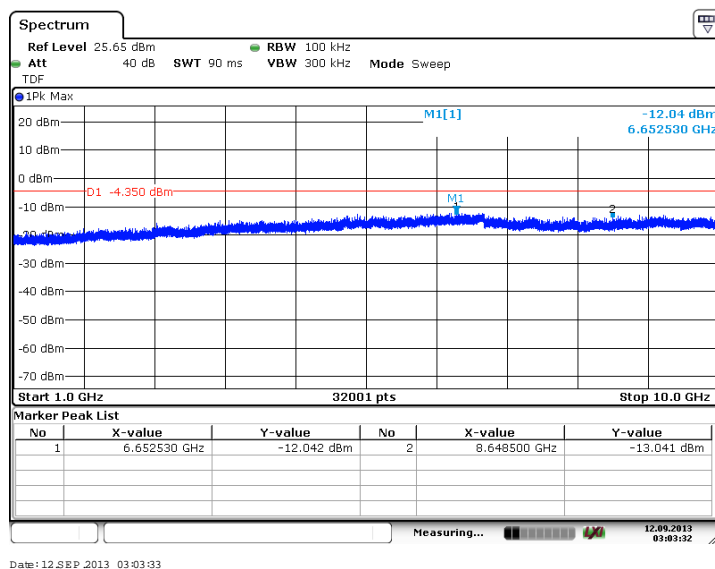
Figure 7.4.2.2-40: 1 GHz – 10 GHz – Middle Channel (64-QAM, Antenna Path 1)
