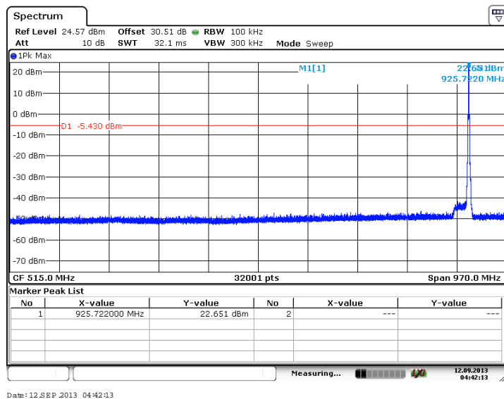
Figure 7.4.2.2-47: 30 MHz – 1 GHz – High Channel (64-QAM, Antenna Path 2)
