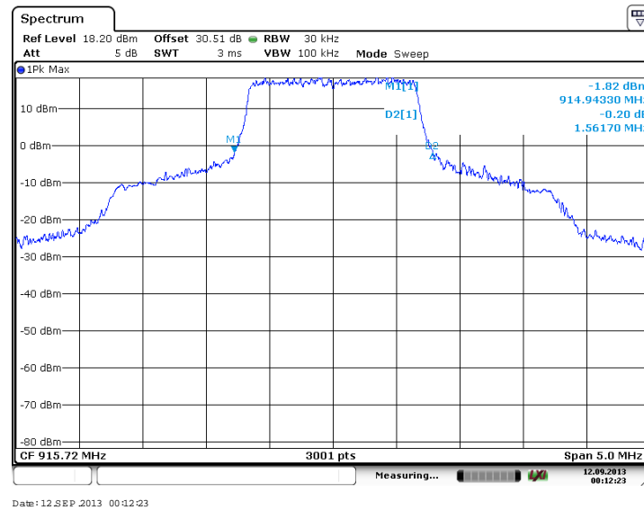
Figure 7.2.2-35: 20 dB OBW - Middle Channel (16-QAM, Antenna Path 2)
