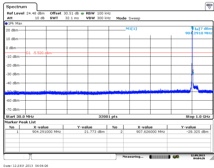
Figure 7.4.2.2-7: 30 MHz – 1 GHz – Low Channel (BPSK, Antenna Path 2)
