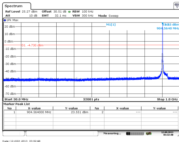
Figure 7.4.2.2-1: 30 MHz – 1 GHz – Low Channel (BPSK, Antenna Path 1)
