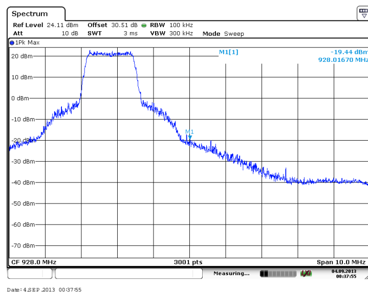
Figure 7.4.1.2-6: Upper Band-edge (QPSK, Antenna Path 1)
