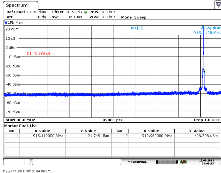
Figure 7.4.2.2-9: 30 MHz – 1 GHz – Middle Channel (BPSK, Antenna Path 2)
