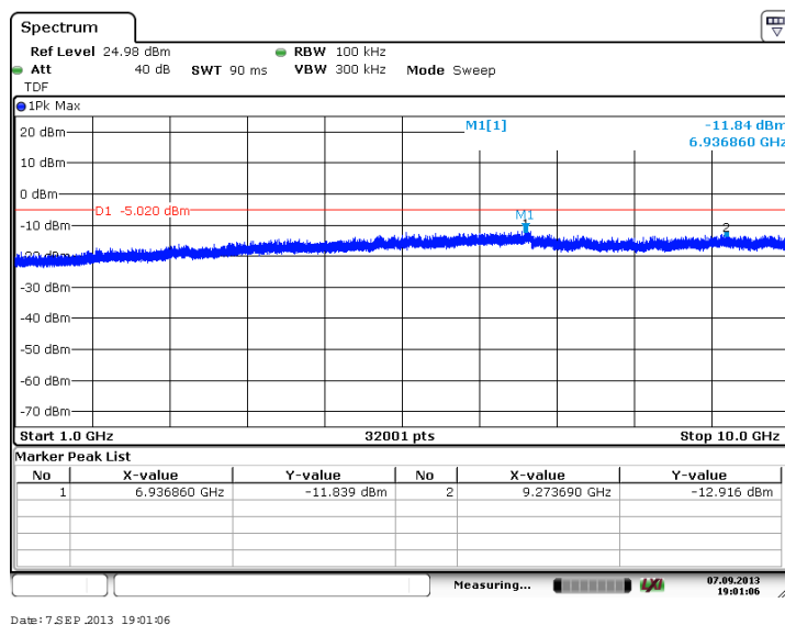
Figure 7.4.2.2-16: 1 GHz – 10 GHz – Middle Channel (QPSK, Antenna Path 1)
