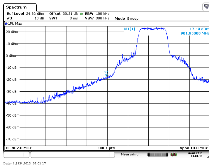
Figure 7.4.1.2-9: Lower Band-edge (16-QAM, Antenna Path 1)
