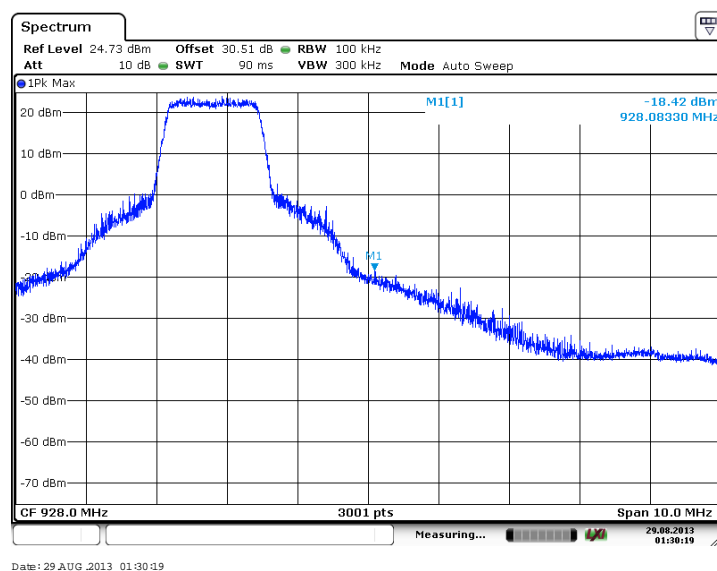
Figure 7.4.1.2-14: Upper Band-edge (64-QAM, Antenna Path 1)
