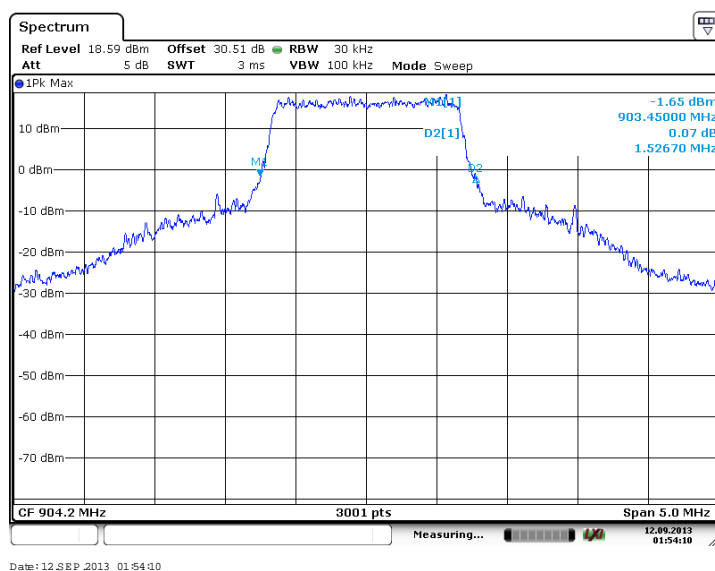
Figure 7.2.2-16: 20 dB OBW - Low Channel (QPSK, Antenna Path 1)
