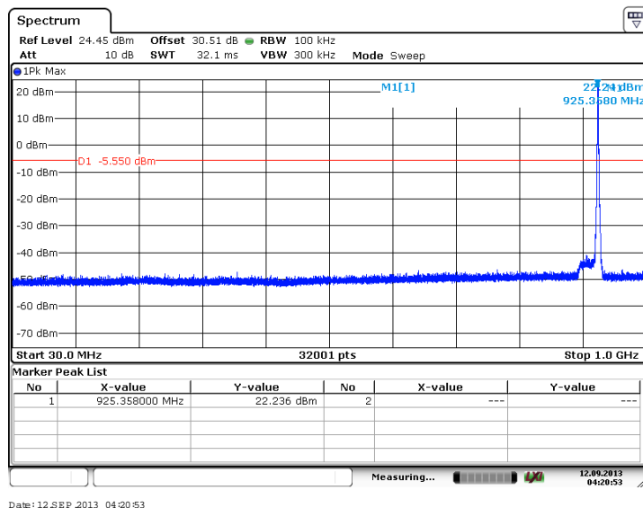
Figure 7.4.2.2-23: 30 MHz – 1 GHz – High Channel (QPSK, Antenna Path 2)
