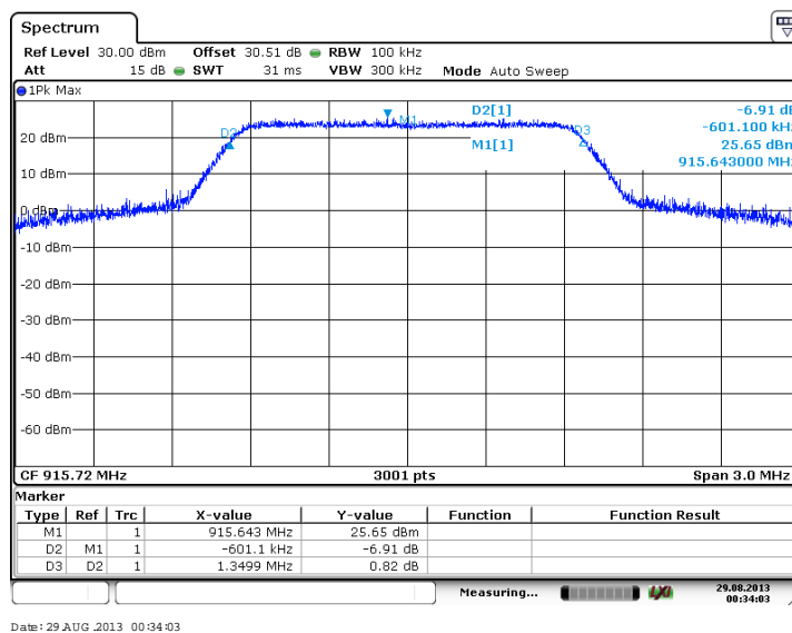
Figure 7.2.2-38: 6dB BW - Middle Channel (64-QAM, Antenna Path 1)
