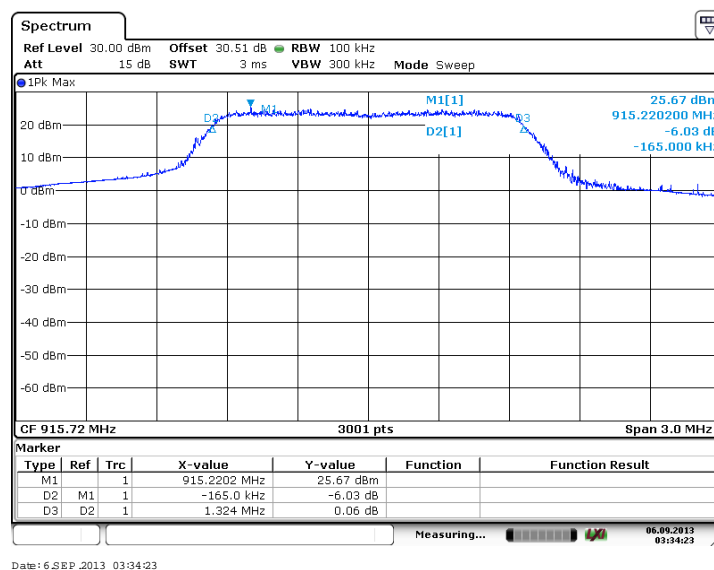
Figure 7.2.2-20: 6dB BW - Middle Channel (QPSK, Antenna Path 2)
