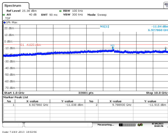
Figure 7.4.2.2-20: 1 GHz – 10 GHz – Low Channel (QPSK, Antenna Path 2)
