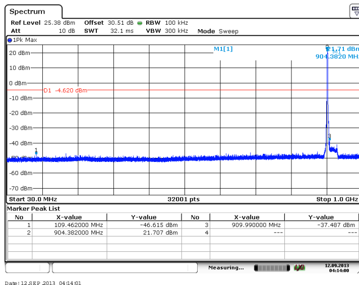
Figure 7.4.2.2-19: 30 MHz – 1 GHz – Low Channel (QPSK, Antenna Path 2)
