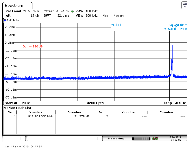
Figure 7.4.2.2-21: 30 MHz – 1 GHz – Middle Channel (QPSK, Antenna Path 2)
