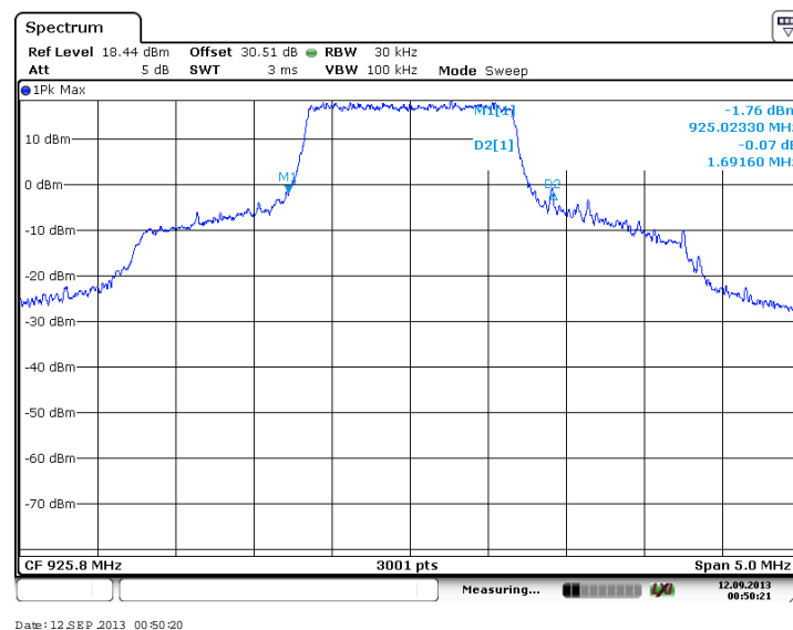
Figure 7.2.2-48: 20 dB OBW - High Channel (64-QAM, Antenna Path 2)
