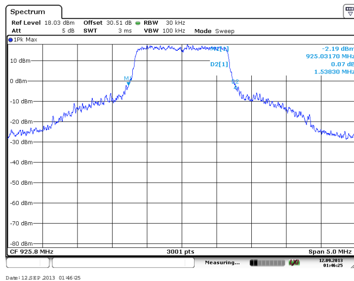
Figure 7.2.2-6: 20 dB OBW - High Channel (BPSK, Antenna Path 1)
