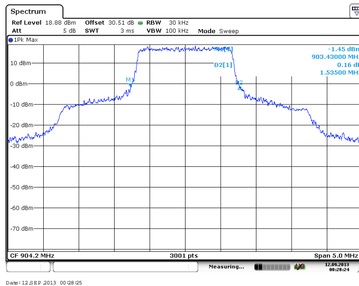
Figure 7.2.2-46: 20 dB OBW - Low Channel (64-QAM, Antenna Path 2)
