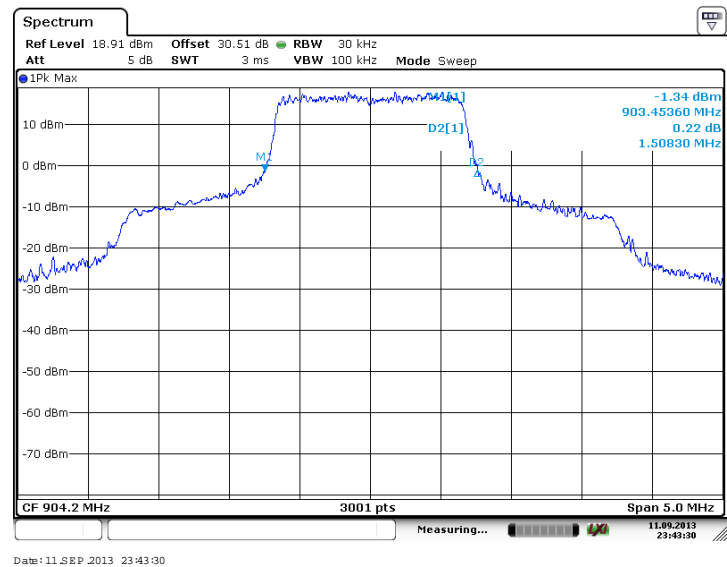
Figure 7.2.2-22: 20 dB OBW - Low Channel (QPSK, Antenna Path 2)
