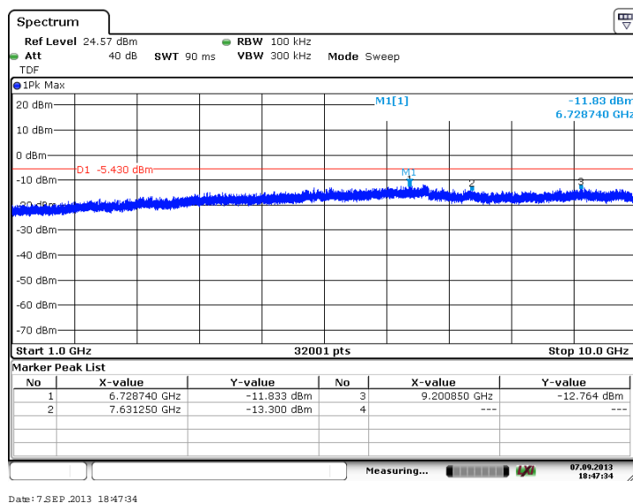
Figure 7.4.2.2-48: 1 GHz – 10 GHz – High Channel (64-QAM, Antenna Path 2)
