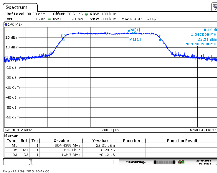
Figure 7.2.2-37: 6dB BW - Low Channel (64-QAM, Antenna Path 1)
