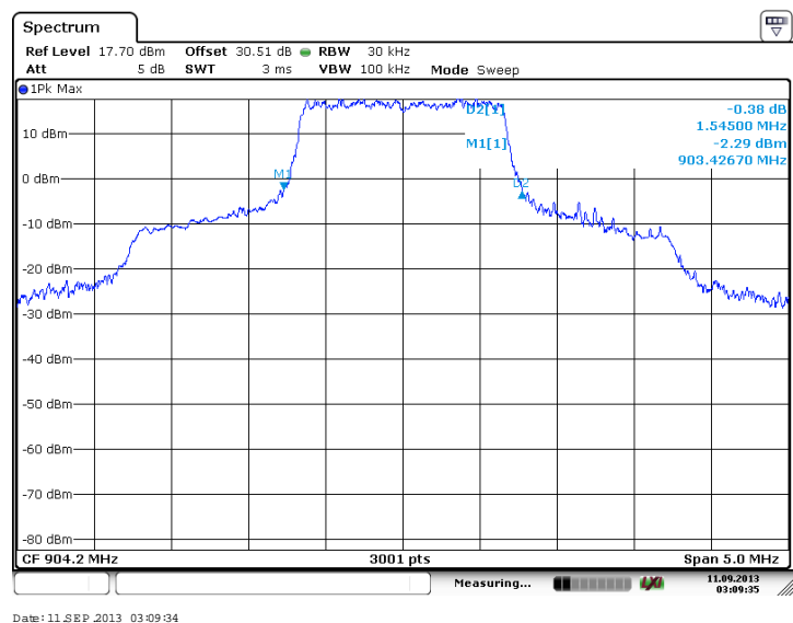
Figure 7.2.2-10: 20 dB OBW - Low Channel (BPSK, Antenna Path 2)
