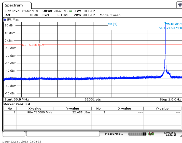
Figure 7.4.2.2-25: 30 MHz – 1 GHz – Low Channel (16-QAM, Antenna Path 1)
