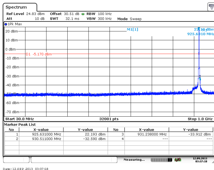
Figure 7.4.2.2-5: 30 MHz – 1 GHz – High Channel (BPSK, Antenna Path 1)
