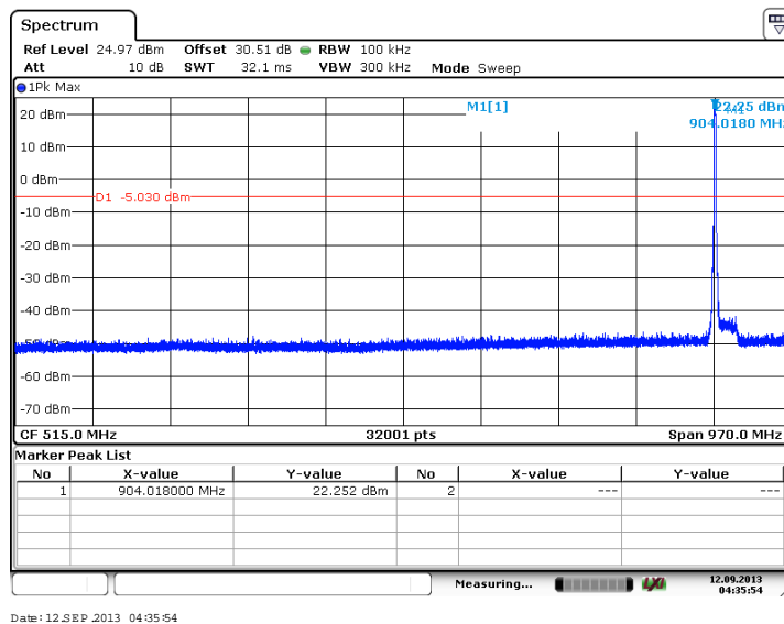
Figure 7.4.2.2-43: 30 MHz – 1 GHz – Low Channel (64-QAM, Antenna Path 2)
