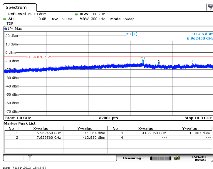
Figure 7.4.2.2-46: 1 GHz – 10 GHz – Middle Channel (64-QAM, Antenna Path 2)
