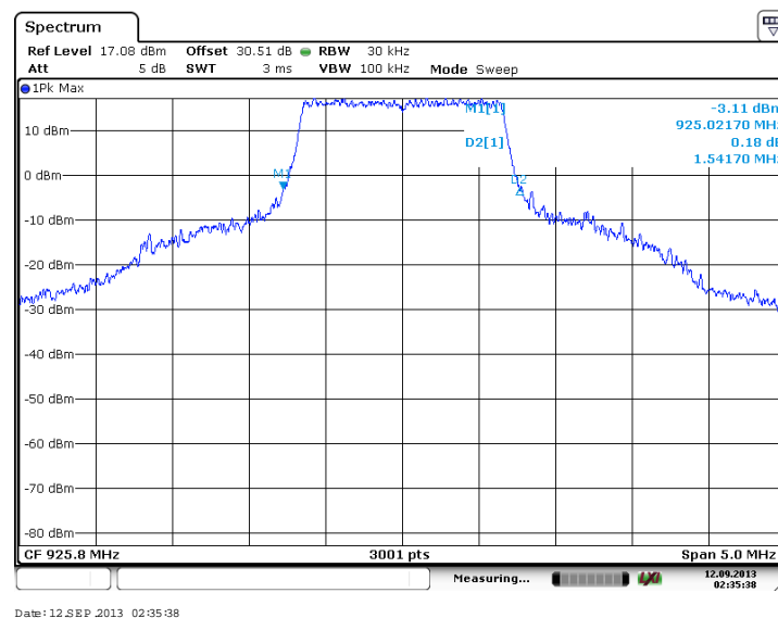
Figure 7.2.2-42: 20 dB OBW - High Channel (64-QAM, Antenna Path 1)
