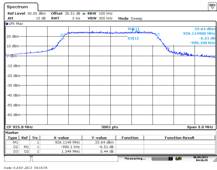
Figure 7.2.2-33: 6dB BW - High Channel (16-QAM, Antenna Path 2)
