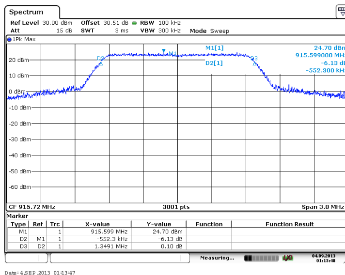
Figure 7.2.2-26: 6dB BW - Middle Channel (16-QAM, Antenna Path 1)
