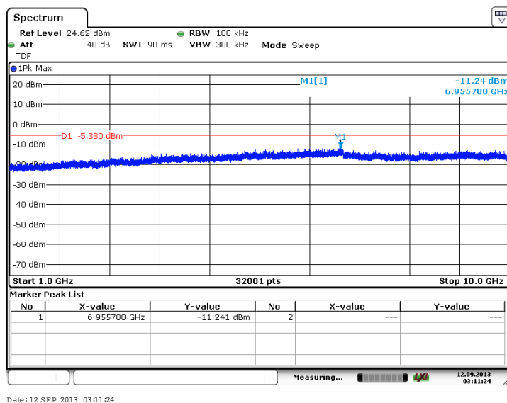
Figure 7.4.2.2-26: 1 GHz – 10 GHz – Low Channel (16-QAM, Antenna Path 1)
