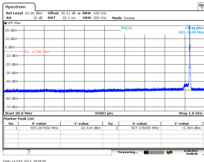
Figure 7.4.2.2-11: 30 MHz – 1 GHz – High Channel (BPSK, Antenna Path 2)
