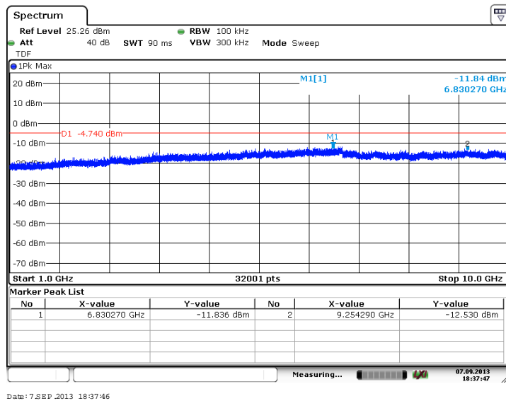
Figure 7.4.2.2-12: 1 GHz – 10 GHz – High Channel (BPSK, Antenna Path 2)
