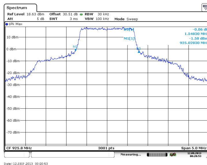
Figure 7.2.2-36: 20 dB OBW - High Channel (16-QAM, Antenna Path 2)
