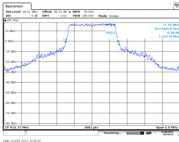
Figure 7.2.2-5: 20 dB OBW - Middle Channel (BPSK, Antenna Path 1)
