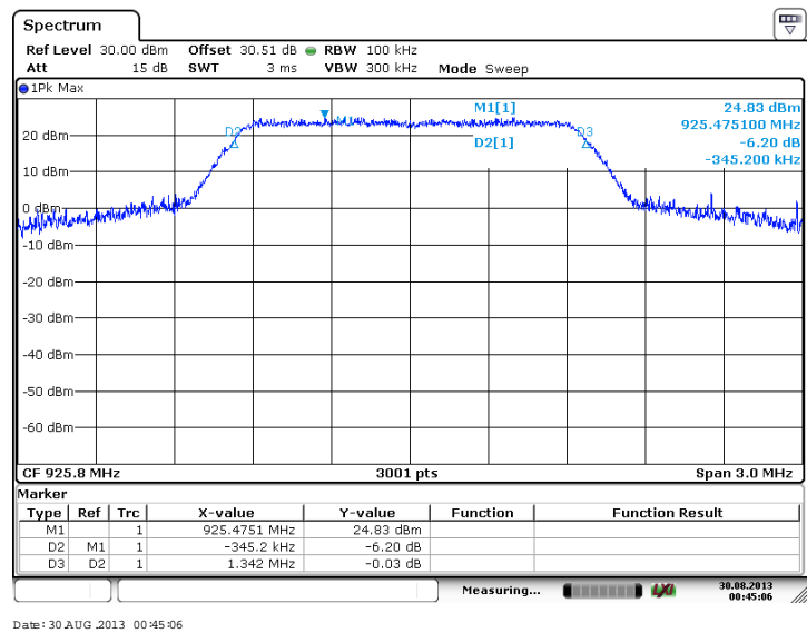
Figure 7.2.2-3: 6dB BW - High Channel (BPSK, Antenna Path 1)
