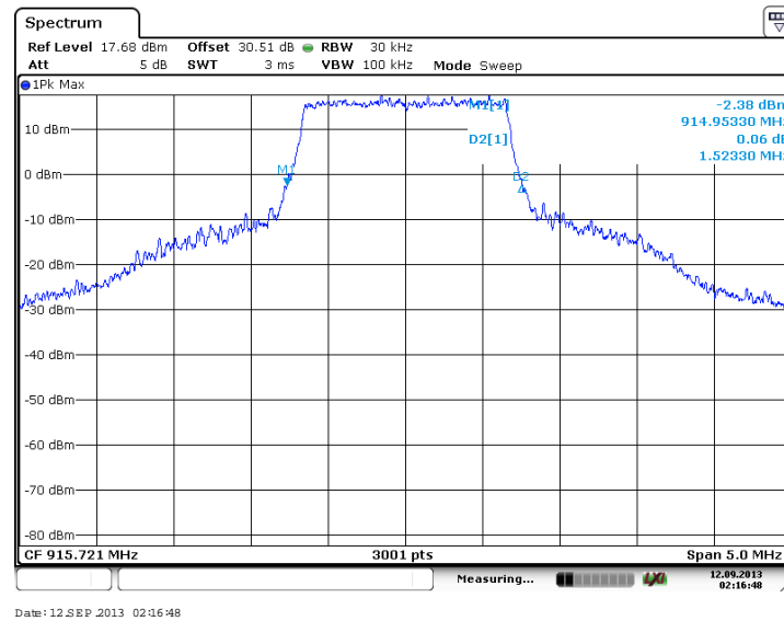
Figure 7.2.2-29: 20 dB OBW - Middle Channel (16-QAM, Antenna Path 1)
