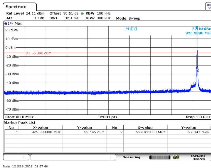
Figure 7.4.2.2-17: 30 MHz – 1 GHz – High Channel (QPSK, Antenna Path 1)
