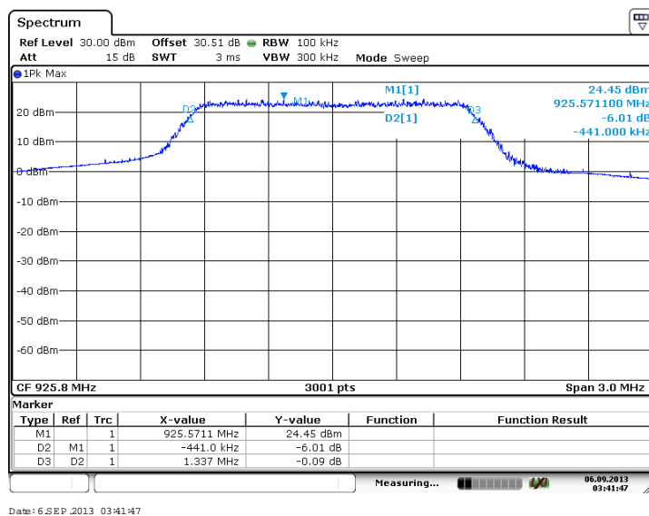
Figure 7.2.2-15: 6dB BW - High Channel (QPSK, Antenna Path 1)
