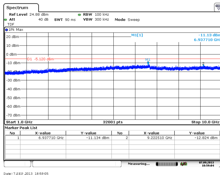
Figure 7.4.2.2-14: 1 GHz – 10 GHz – Low Channel (QPSK, Antenna Path 1)
