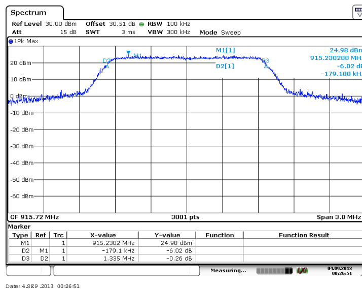
Figure 7.2.2-14: 6dB BW - Middle Channel (QPSK, Antenna Path 1)
