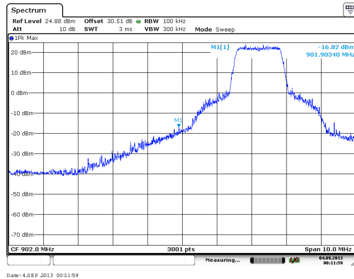
Figure 7.4.1.2-5: Lower Band-edge (QPSK, Antenna Path 1)
