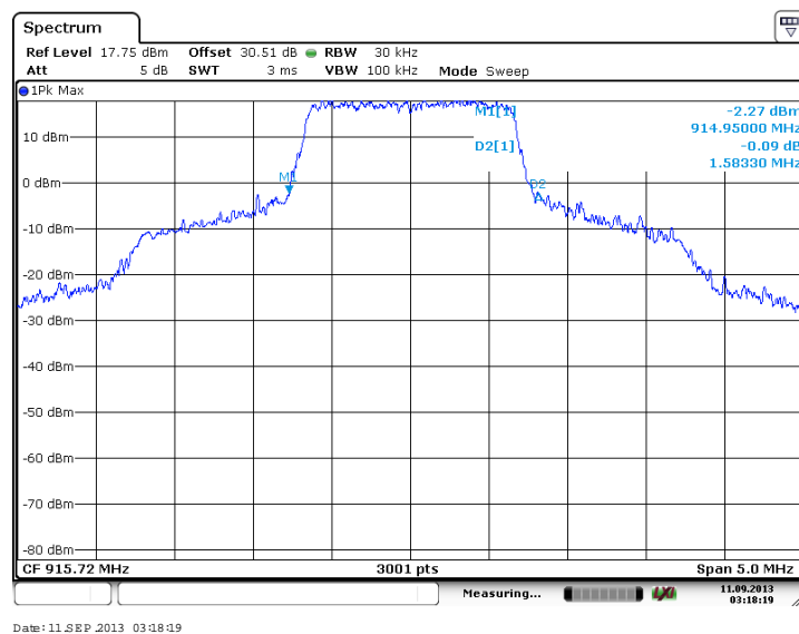
Figure 7.2.2-11: 20 dB OBW - Middle Channel (BPSK, Antenna Path 2)
