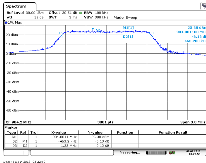
Figure 7.2.2-19: 6dB BW - Low Channel (QPSK, Antenna Path 2)
