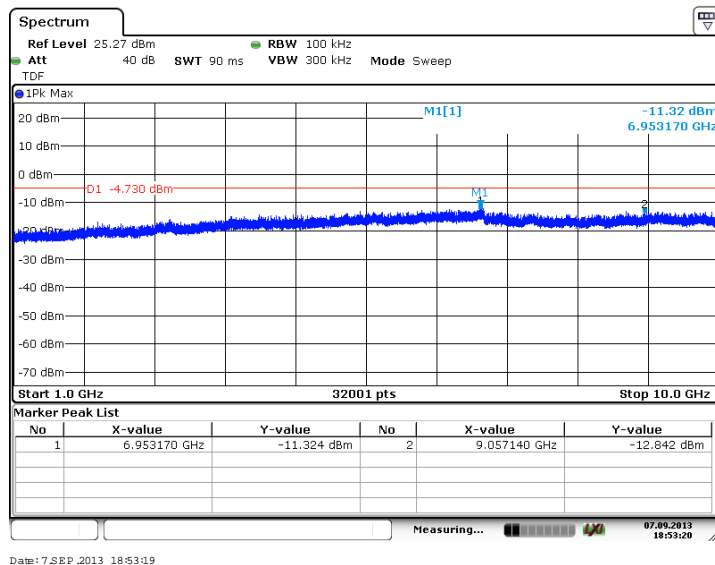
Figure 7.4.2.2-2: 1 GHz – 10 GHz – Low Channel (BPSK, Antenna Path 1)
