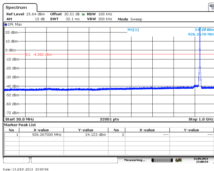
Figure 7.4.2.2-35: 30 MHz – 1 GHz – High Channel (16-QAM, Antenna Path 2)
