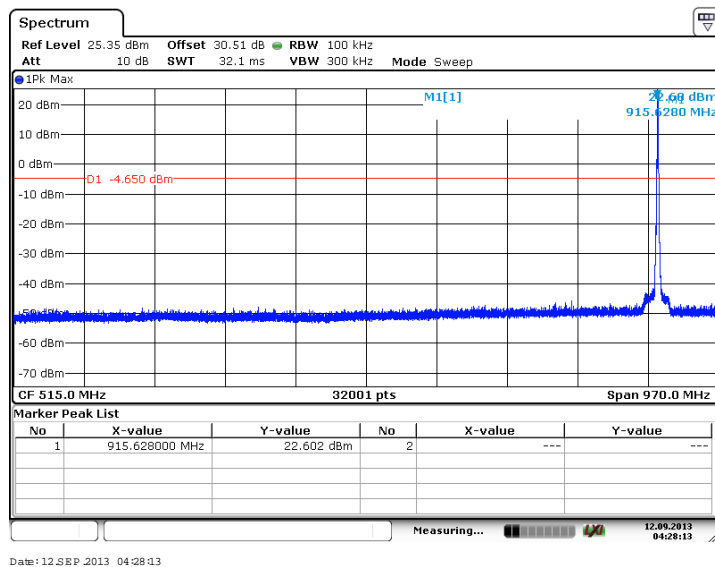
Figure 7.4.2.2-33: 30 MHz – 1 GHz – Middle Channel (16-QAM, Antenna Path 2)
