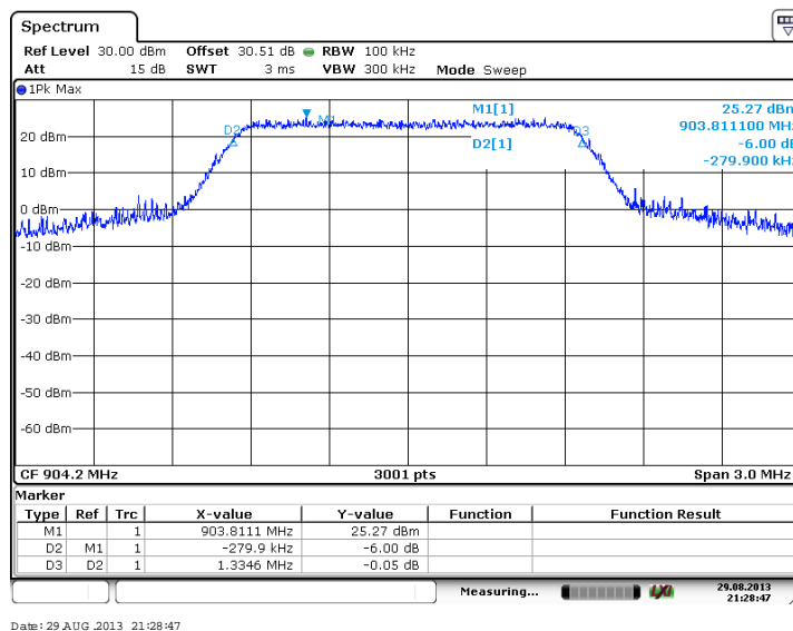
Figure 7.2.2-1: 6dB BW - Low Channel (BPSK, Antenna Path 1)
