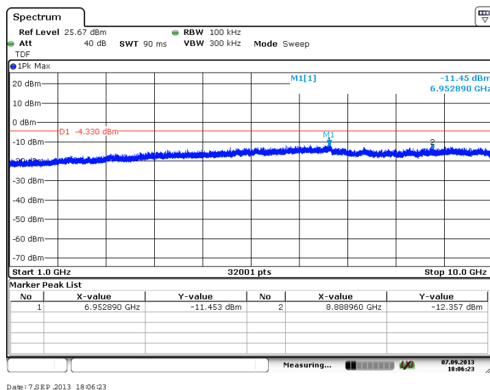
Figure 7.4.2.2-22: 1 GHz – 10 GHz – Middle Channel (QPSK, Antenna Path 2)
