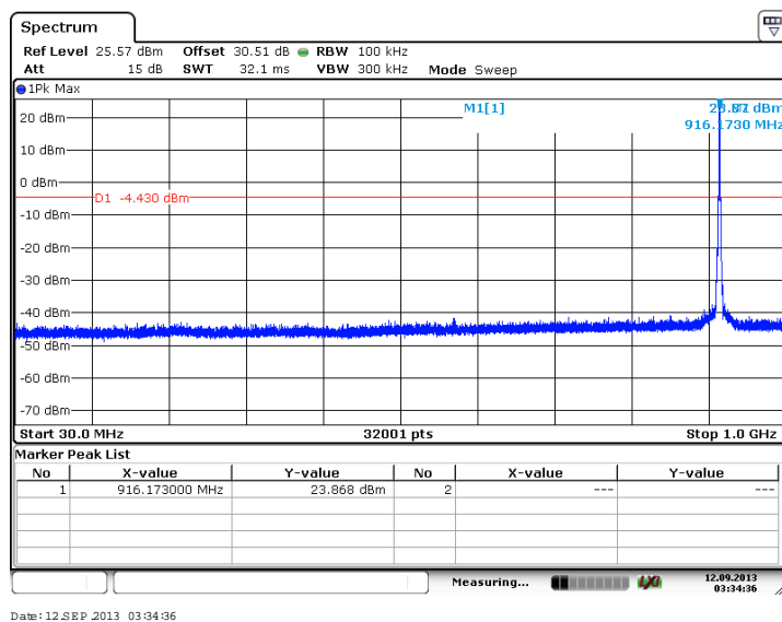
Figure 7.4.2.2-3: 30 MHz – 1 GHz – Middle Channel (BPSK, Antenna Path 1)
