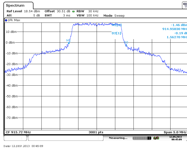
Figure 7.2.2-47: 20 dB OBW - Middle Channel (64-QAM, Antenna Path 2)
