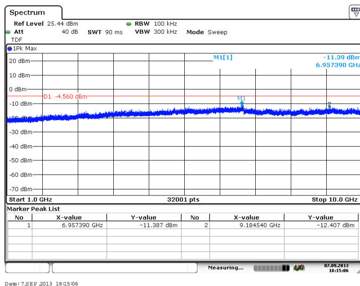
Figure 7.4.2.2-32: 1 GHz – 10 GHz – Low Channel (16-QAM, Antenna Path 2)
