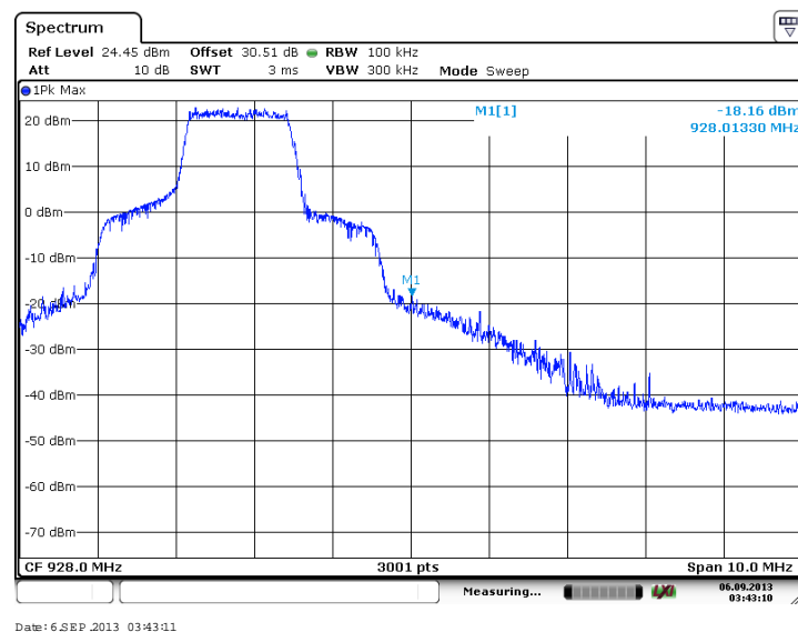
Figure 7.4.1.2-8: Upper Band-edge (QPSK, Antenna Path 2)
