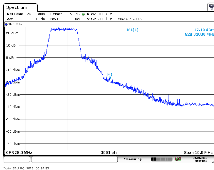
Figure 7.4.1.2-2: Upper Band-edge (BPSK, Antenna Path 1)
