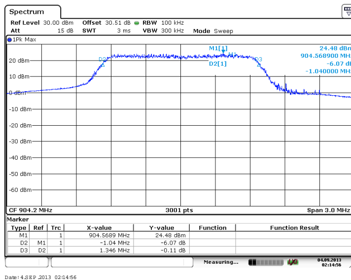
Figure 7.2.2-7: 6dB BW - Low Channel (BPSK, Antenna Path 2)
