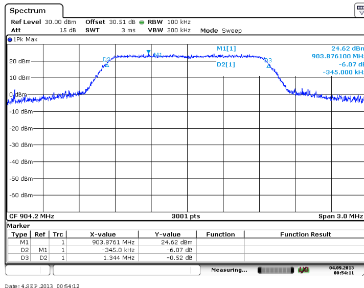
Figure 7.2.2-25: 6dB BW - Low Channel (16-QAM, Antenna Path 1)
