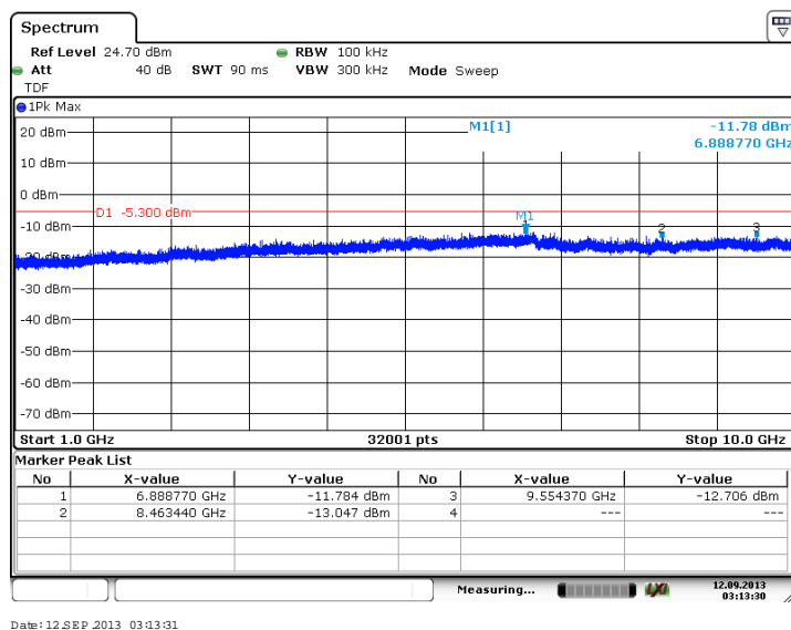
Figure 7.4.2.2-28: 1 GHz – 10 GHz – Middle Channel (16-QAM, Antenna Path 1)
