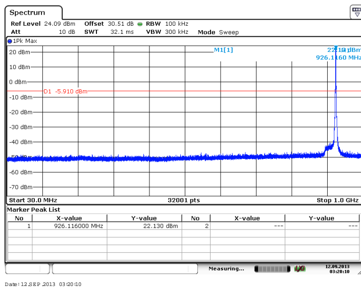
Figure 7.4.2.2-29: 30 MHz – 1 GHz – High Channel (16-QAM, Antenna Path 1)
