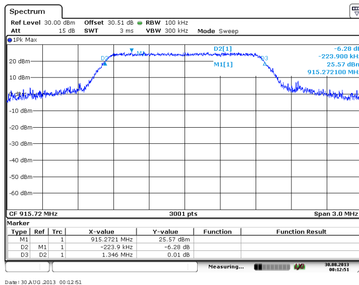
Figure 7.2.2-2: 6dB BW - Middle Channel (BPSK, Antenna Path 1)
