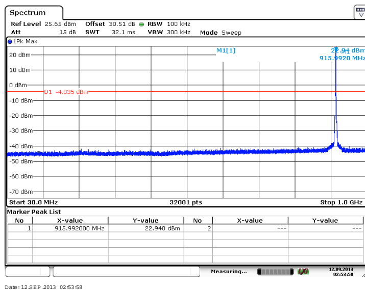
Figure 7.4.2.2-39: 30 MHz – 1 GHz – Middle Channel (64-QAM, Antenna Path 1)
