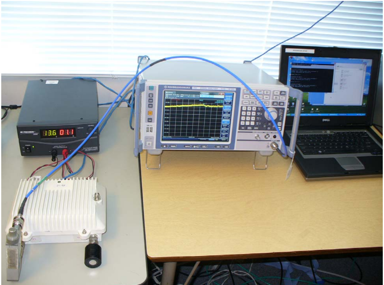
Figure 3: RF Conducted
