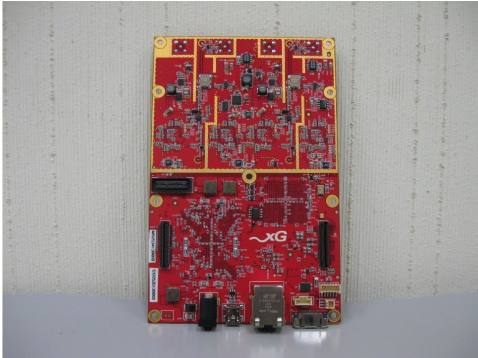
Fig-1. xModem Main Board Top View
