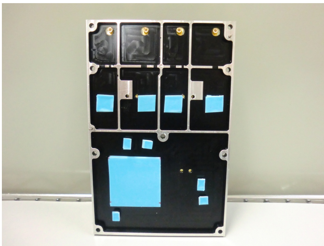
Fig-6. xModem Antenna Heat Sink Internal view
