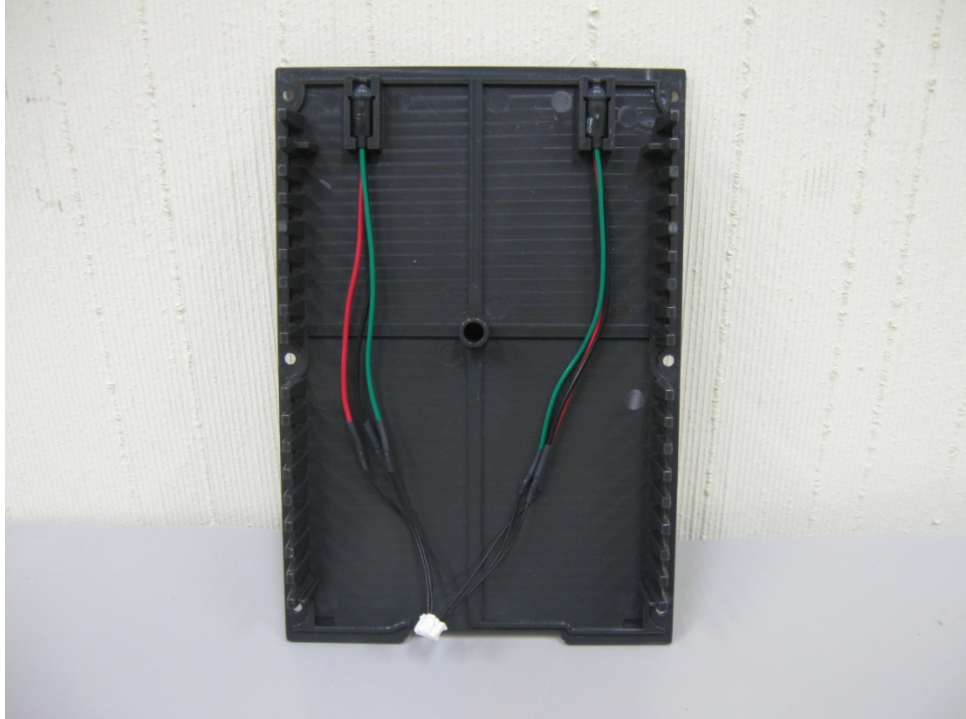
Fig-19. xModem Bottom Cover with LED Assembly
