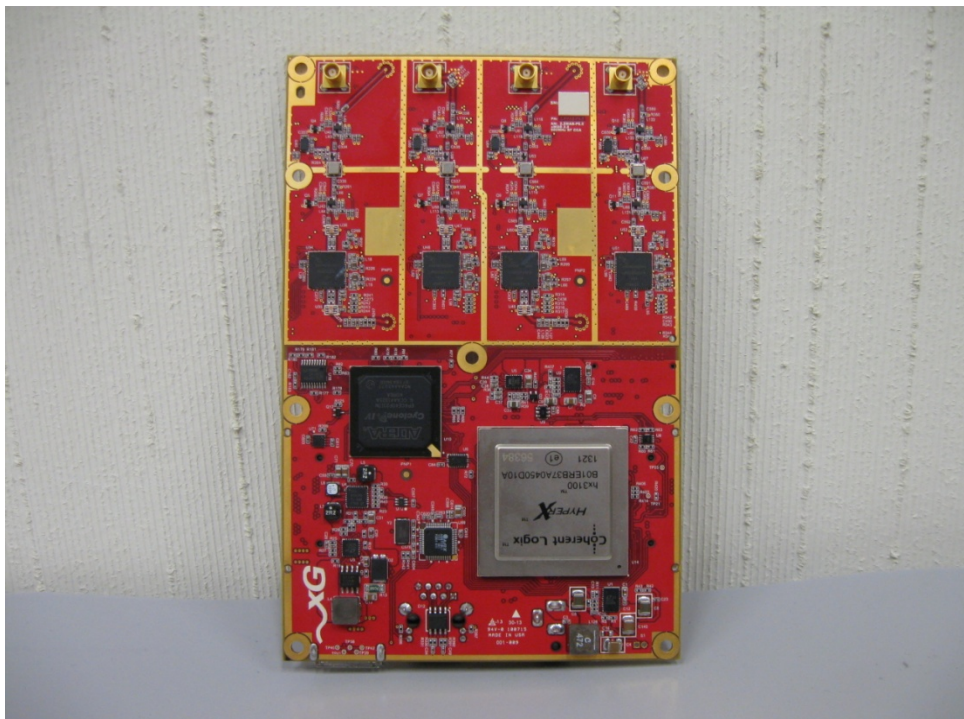
Fig-2. xModem Main Board Bottom View
