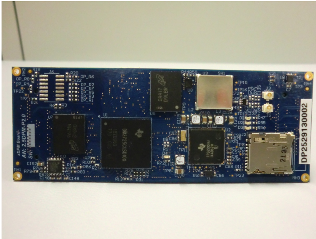
Fig-3. DPM Board Top View
