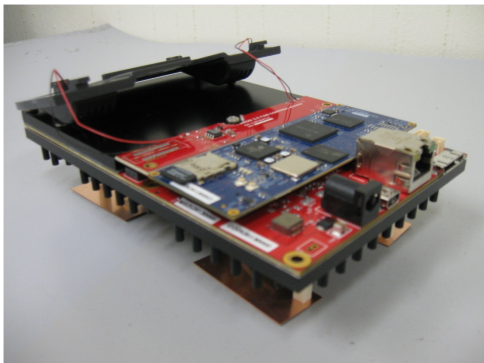
Fig-14. xModem Assembly Side View
