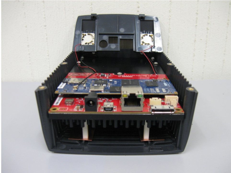
Fig-17. xModem Assembly inside Top Housing. Side View
