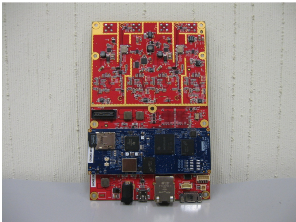
Fig-5. Main Board and DPM Assembly
