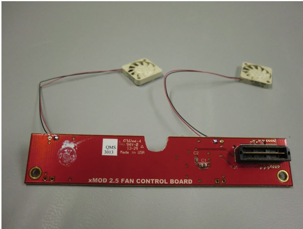
Fig-11. xModem Fan Control Board Bottom View
