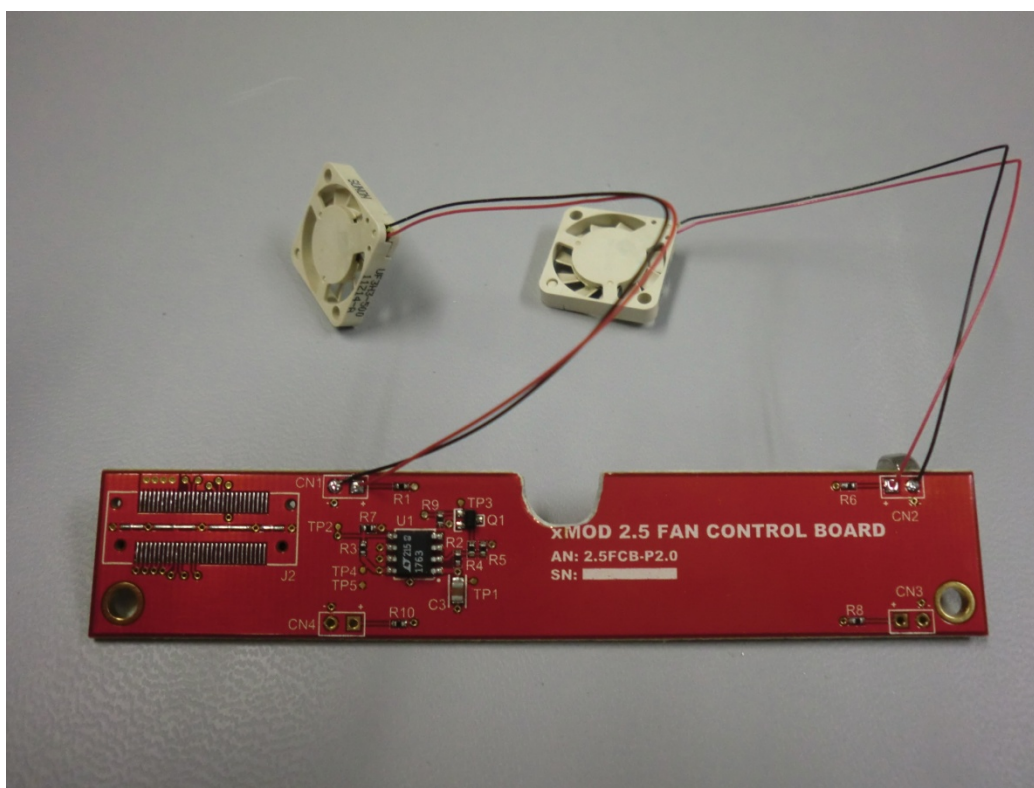
Fig-10. xModem Fan Control Board Top View
