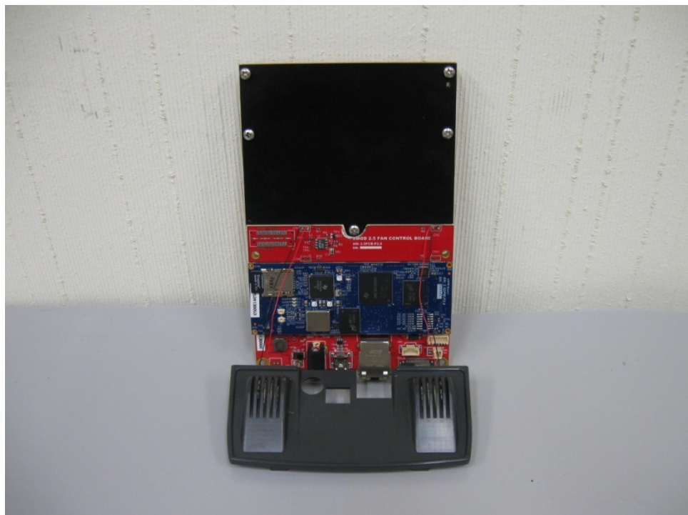
Fig-12. xModem Assembly Top View
