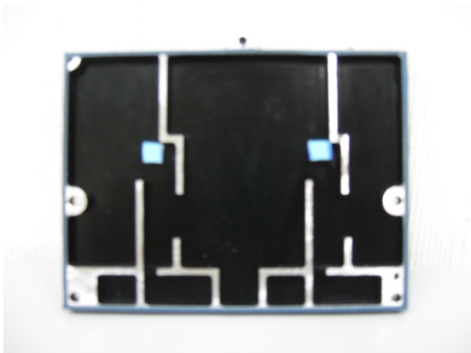
Fig-8. xModem RF Shield Internal view w/Thermal Pads
